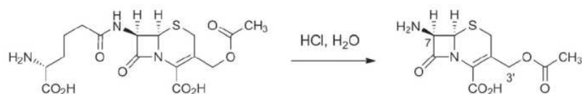
Scheme 1. Hydrolysis of cephalosporin C under acidic conditions
