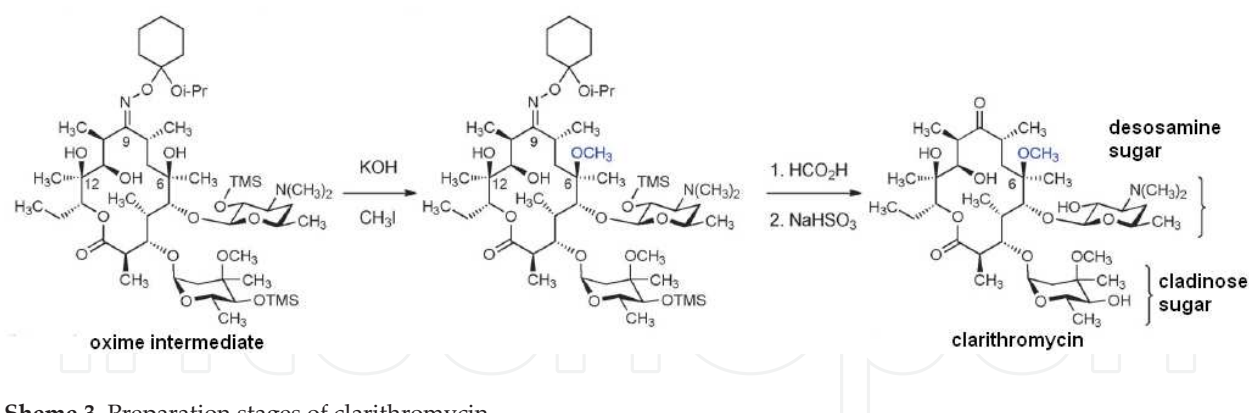
Scheme 3. Preparation stages of clarithromycin
