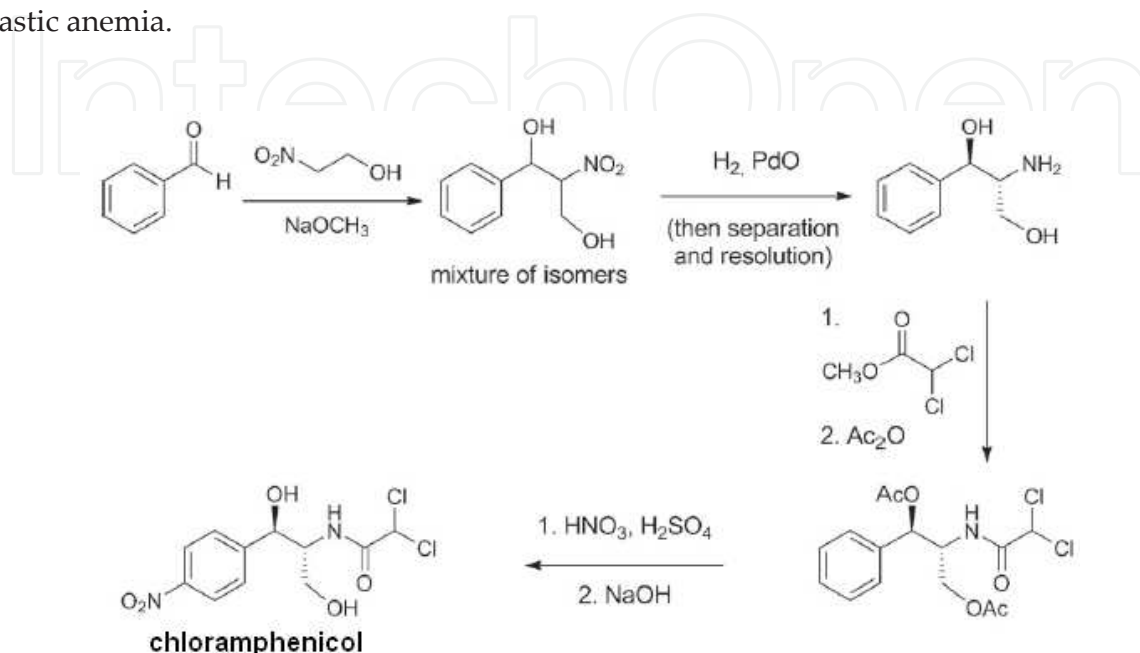
Scheme 4. Synthesis reactions leading to chloramphenicol
