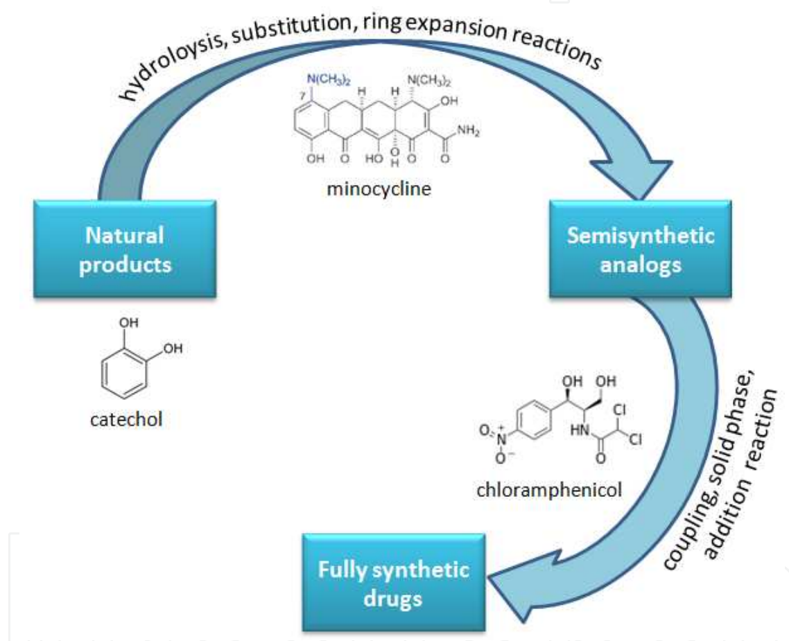
Figure 3. The schematic representation of the main synthesis routes of the antibacterial agents
