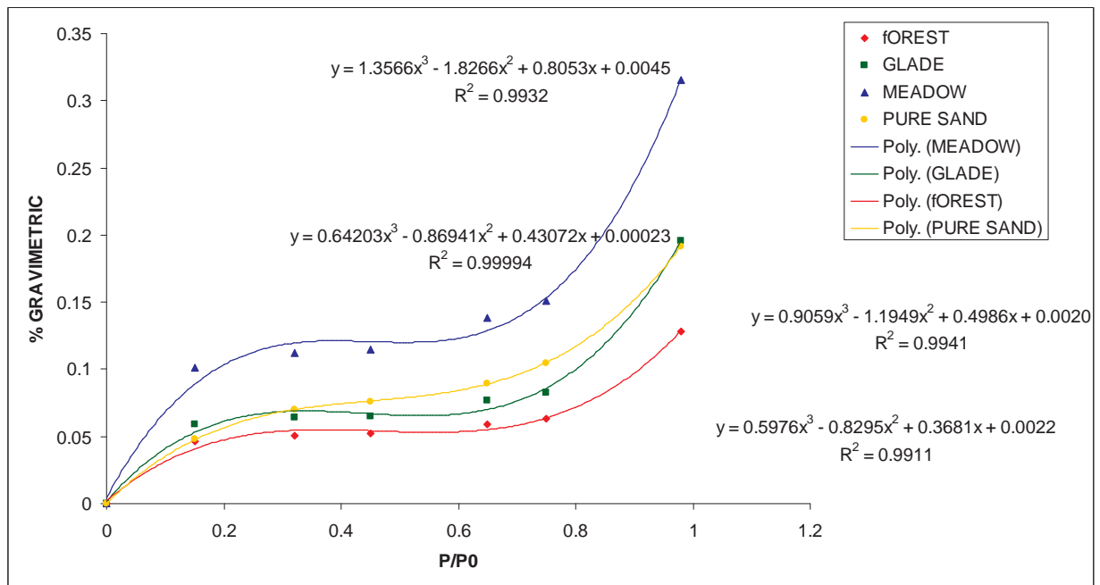
Figure 1. Unpublished data of the relationship between gravimetric adsorbed water (W%) and vapor pressure P/Po in sandy soils (94% sand in average) with plant cover.
