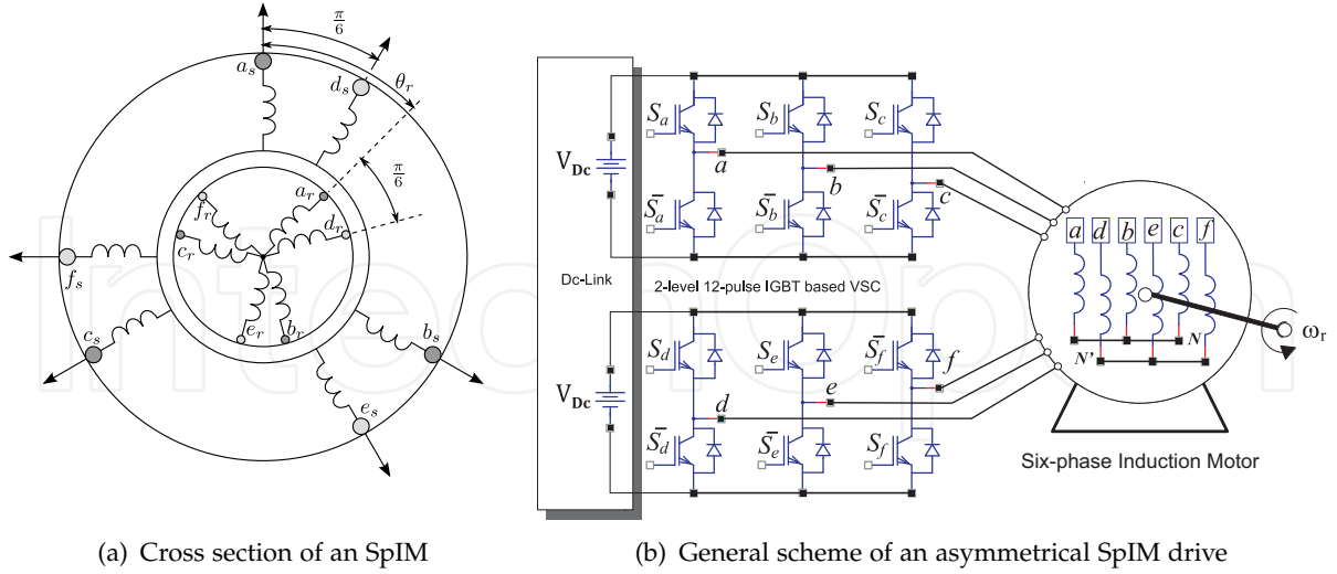
Figure 1. Asymmetrical SpIM feed topology and winding configuration
