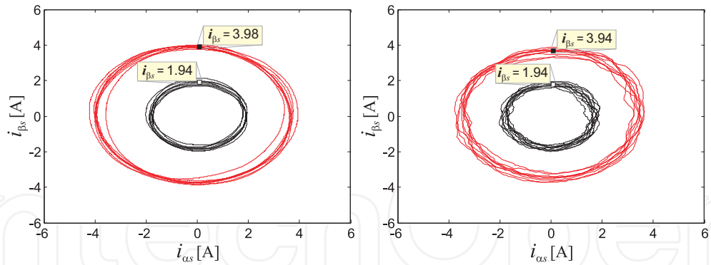
(a) i_{\alpha s} vs. i_{\beta s} current obtained by using the (b) i_{\alpha s} vs. i_{\beta s} current obtained by experimental MatLab/Simulink simulation environment tests
