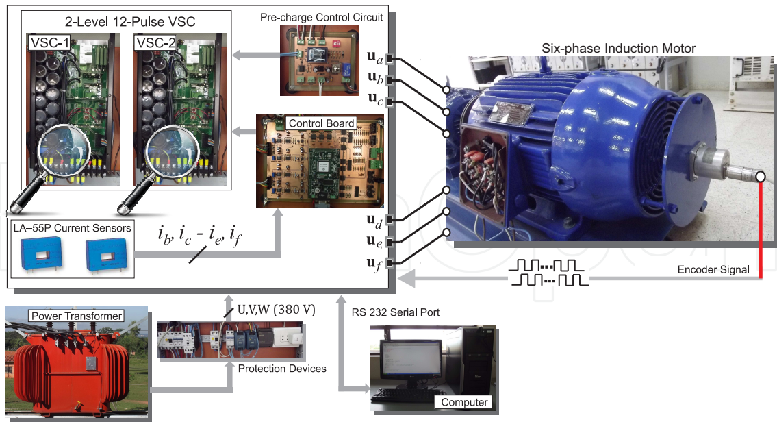
Figure 3. Scheme of the experimental setup
