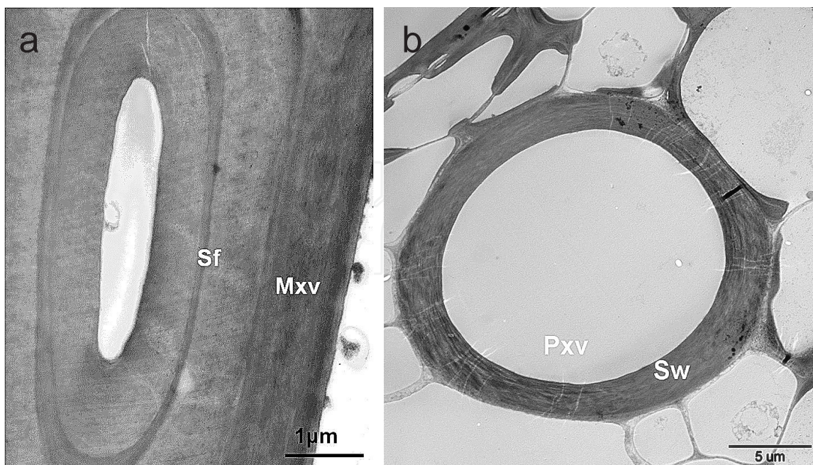
Figure 6. TEM images showing layering structure of Miscanthus sinensis internode tissue. (a) Metaxylem vessel (Mxv); (b) protoxylem vessel (Pxv).
