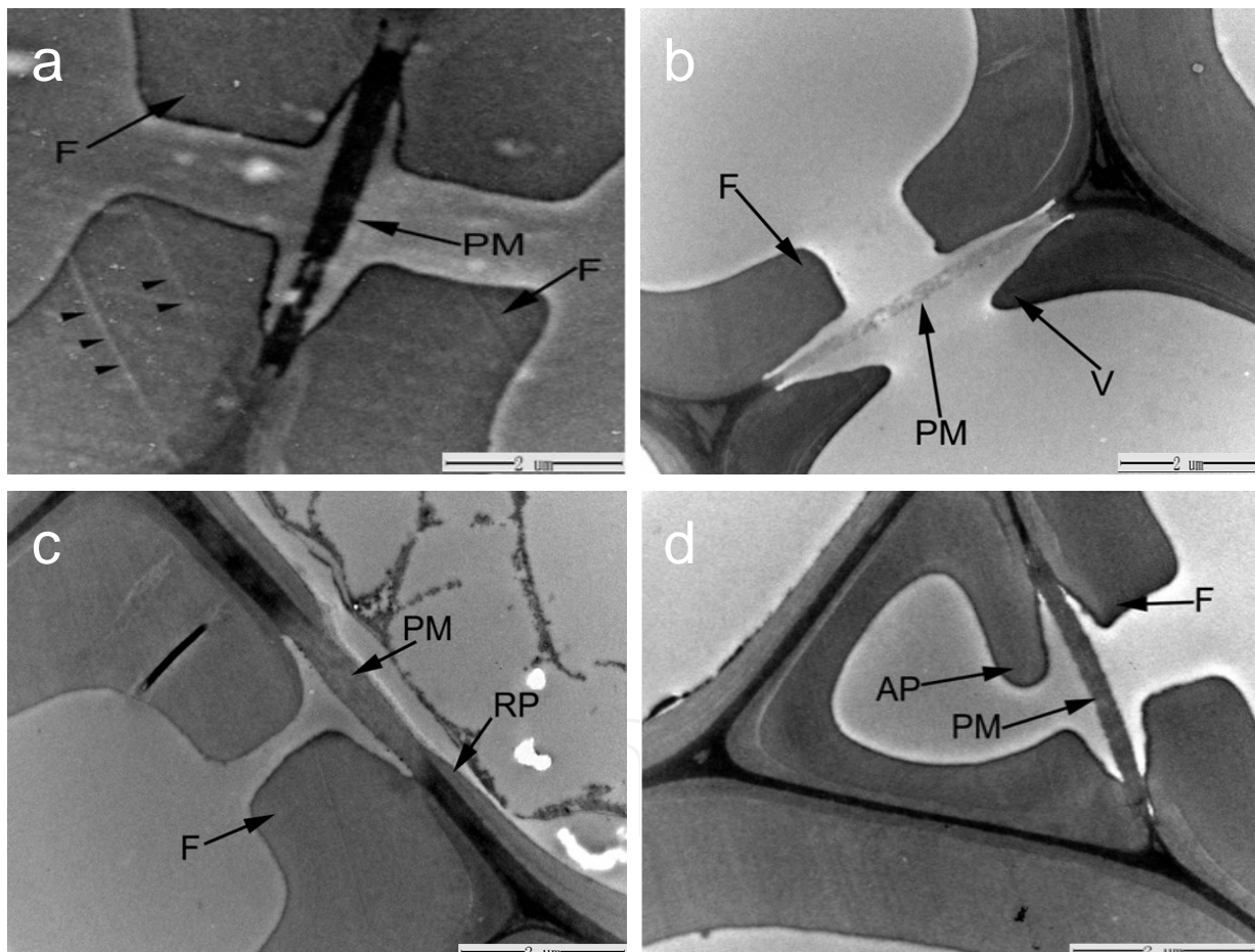
Figure 2. TEM micrographs of pit membrane among various cells in C. alba L. , taken at 80 kV. (a) Pit membrane between fibers, (arrowheads: knife mark). (b) Pit membrane between fiber and vessel. (c) Pit membrane between fiber and ray parenchyma. (d) Pit membrane between fiber and axial parenchyma. F, fiber; V, vessel; RP, ray parenchyma; AP, axial parenchyma; PM, pit membrane.
