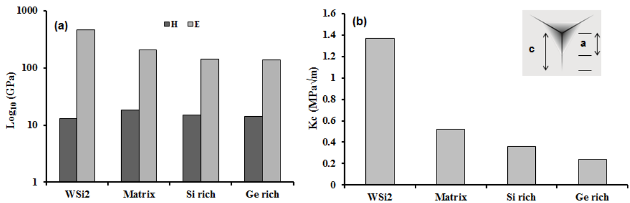
Figure 14. (a) Quantitative results for H and E for all phases. (b) k_c values for all phases. The inset is a schematic of radial crack formation induced by nanoindentation. Reproduced from reference 18 with permission from Elsevier.
