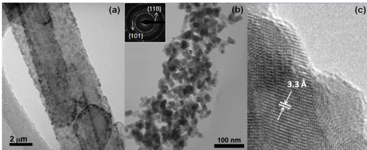
Figure 9. (a) TEM image of MWCNT covered with SnO 2 nanoparticles. (b) TEM image of a porous SnO 2 nanorod. Inset shows the ED pattern. (c) HRTEM image showing that the lattice spacing corresponds to the rutile structure of SnO 2 . Reproduced from reference 13 with permission from the Institute of Physics.
