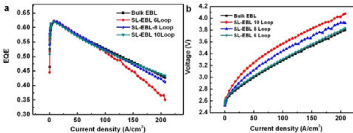
Fig. 4 EQE (a) and I-V (b) characteristics as a function of injection current for the LEDs with Bulk EBL and SL-EBL with different loop numbers.
