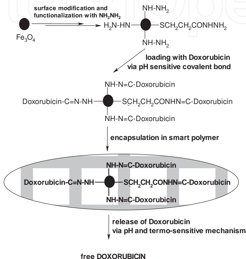
Scheme 5. Synthesis and dual-sensitive magnetic drug delivery system
