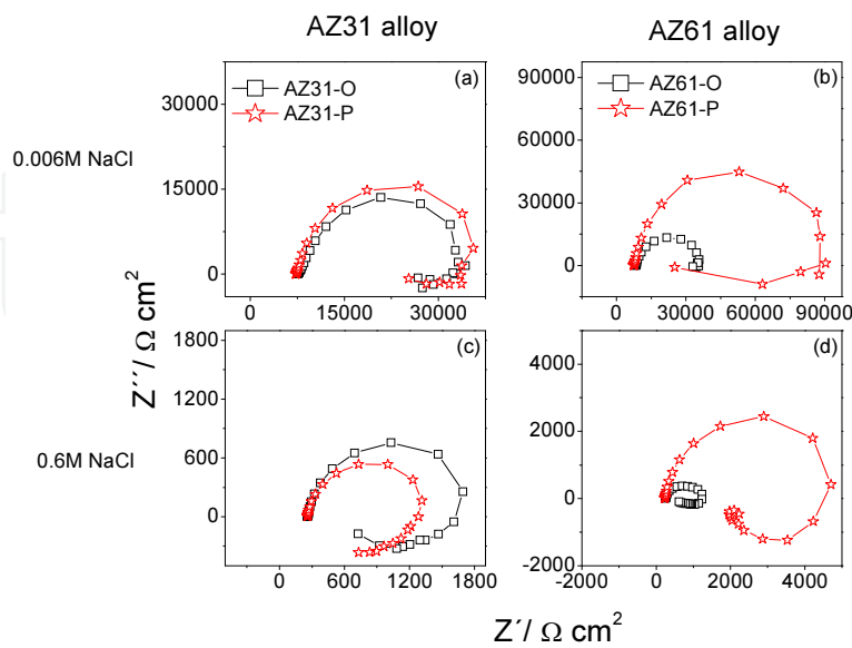
Figure 7. Comparison of the Nyquist plot as a function of substrate surface conditions and alloy type after 1 day of immersion in saline solutions with two different chloride ion concentrations.
