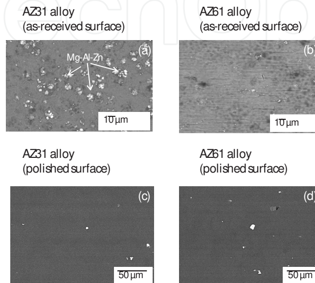
Figure 1. (a, b) SEM morphologies of the surfaces in the AZ31-O and AZ61-O and (c, d) AZ31-P and AZ61-P specimens (figure adapted from [45] and [46]).
