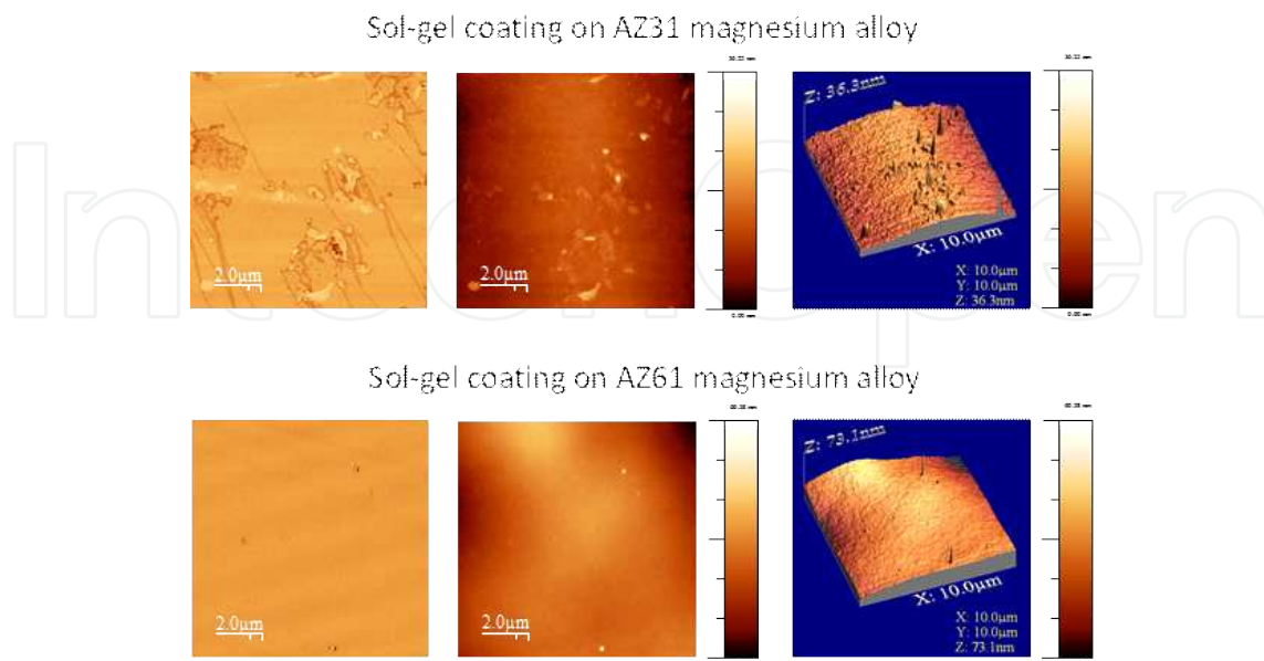
Figure 12. AFM topography images of the sol-gel coating formed on the AZ31 and AZ61 alloys substrates.
