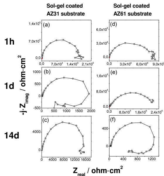
Figure 13. Variation in Nyquist plots as a function of the coated alloy-type substrate during immersion tests in 0.6 M NaCl aqueous solution.
