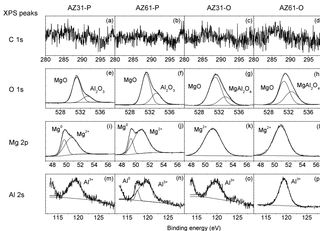
Figure 4. (a-d) Variation in the C1s, (e-h) O1s, (i-l) Mg2p and (m-p) Al2s high-resolution peaks obtained by XPS on the surface of the specimens after 5 min sputtering as a function of surface conditions and alloy type (figure adapted from [27]).
