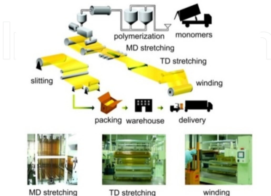
Figure 5. Industrial-scale manufacturing for PI films via PAA precursors
