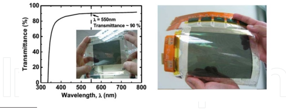
Figure 11. Colorless PI substrate and the color VGA flexible TFT-LCD
