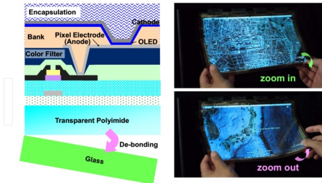
Figure 12. Flexible 10.2-inch AMOLED devices on transparent PI substrates [29]
