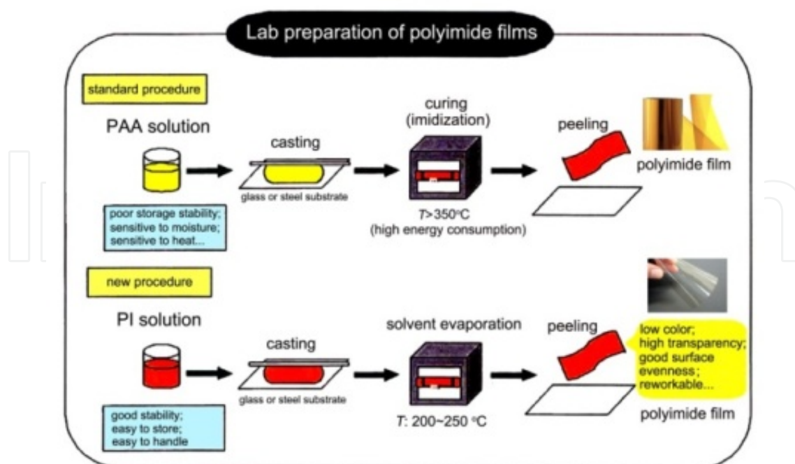
Figure 4. Lab-scale preparation of PI films
