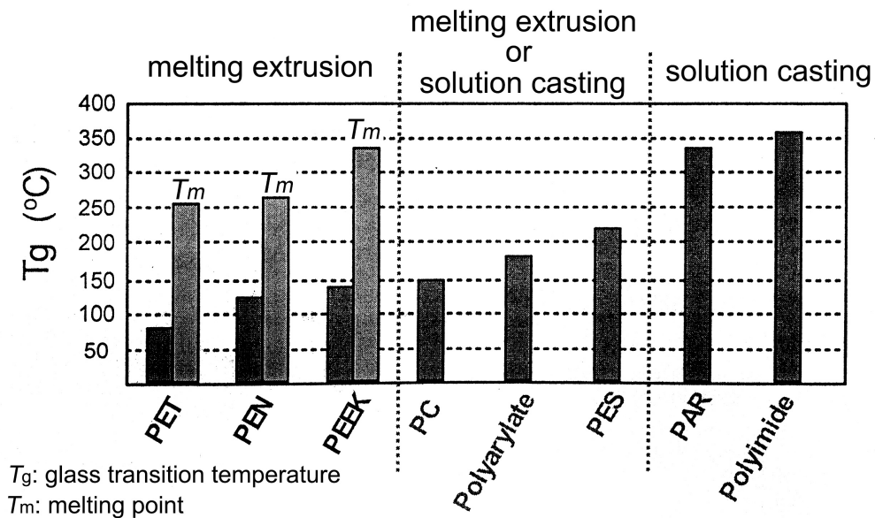
Figure 3. Processing methods for polymer films
