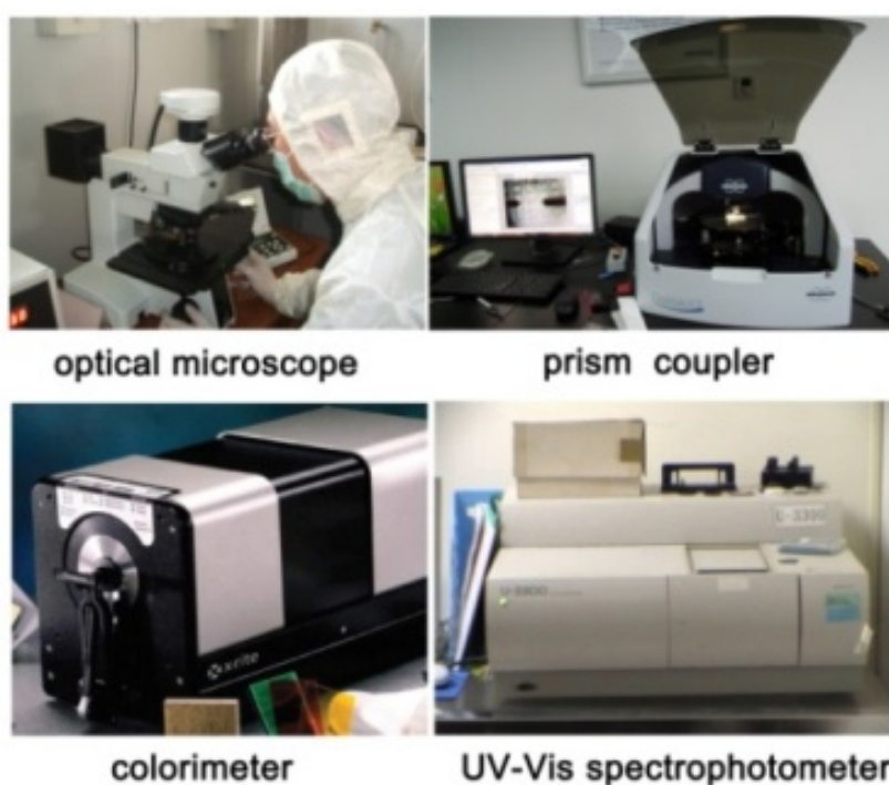
Figure 7. Optical properties measurement system
