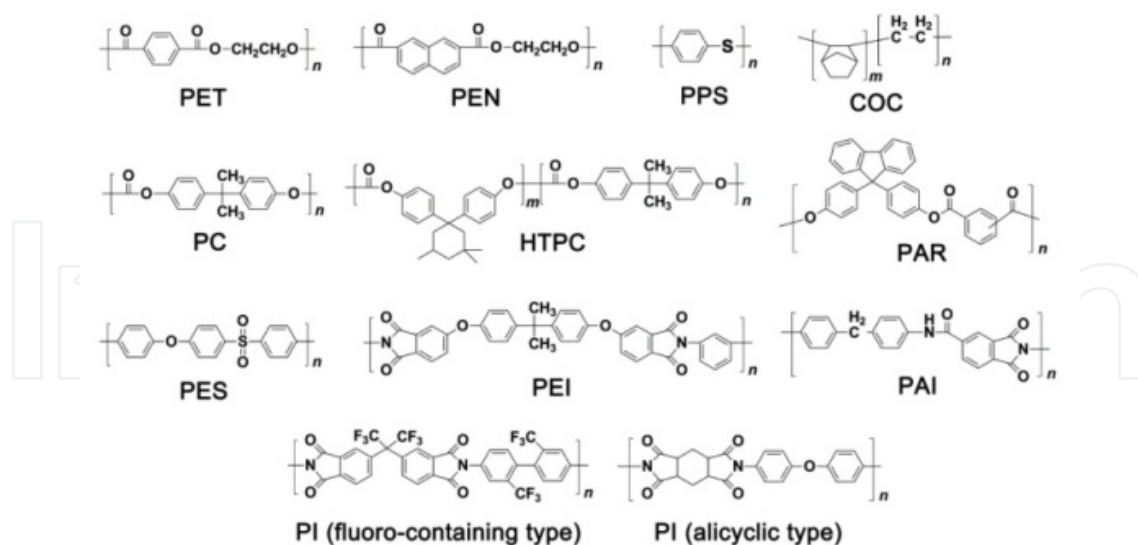
Figure 2. Typical chemical structures for polymer optical films
