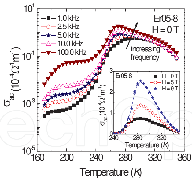
Figure 9. (Color online) Temperature dependence of ac conductivity ( \sigma_{ac} ) of Er05-8 for various frequencies. Inset: temperature dependence of ac conductivity ( \sigma_{ac} ) at 2.5 kHz with external magnetic fields.
