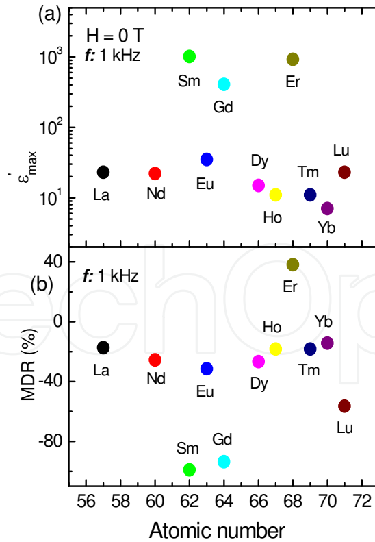
Figure 13. (Color online) (a) Maximum value of dielectric constant, and (b) MDR under 5 T applied field of RE_2O_3:SiO_2 nano-glass composite systems calcined at 700^\circ C with rare earth atomic number.
