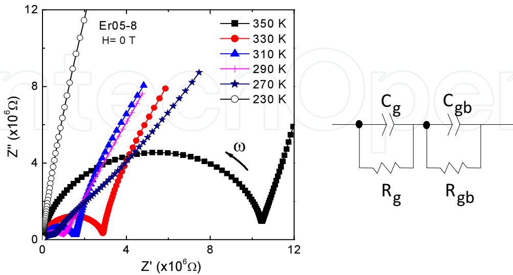
Figure 6. (Color online) (a) Complex plane plots, Z''-Z' , of Er05-8 at several temperatures and (b) schematic model of equivalent electrical circuits indicating of two parallel resistor–capacitor (RC) combinations [ (R_gC_g) : Er 2 O 3 nano-grain, (R_{gb}C_{gb}) : SiO 2 matrix] connected in series.
