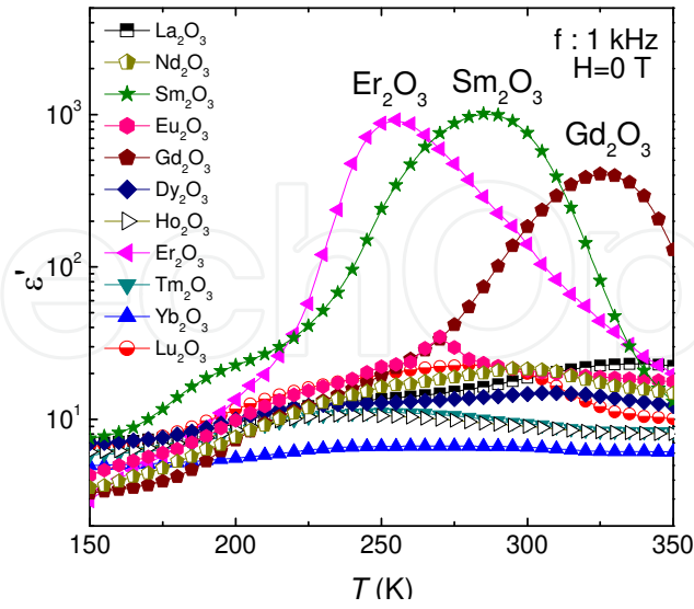
Figure 12. (Color online) The \epsilon' - T curves of RE_2O_3 (gel-glass calcined at 700^\circ C ) at 1 kHz without applied magnetic field.
