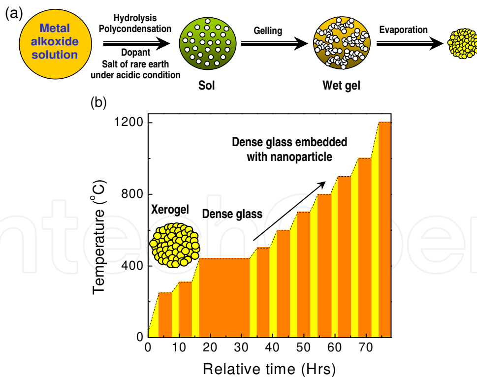
Figure 1. (Color online) (a) Sol-gel process. (b) Gel-glass embedded with rare earth nanoparticle calcination process.
