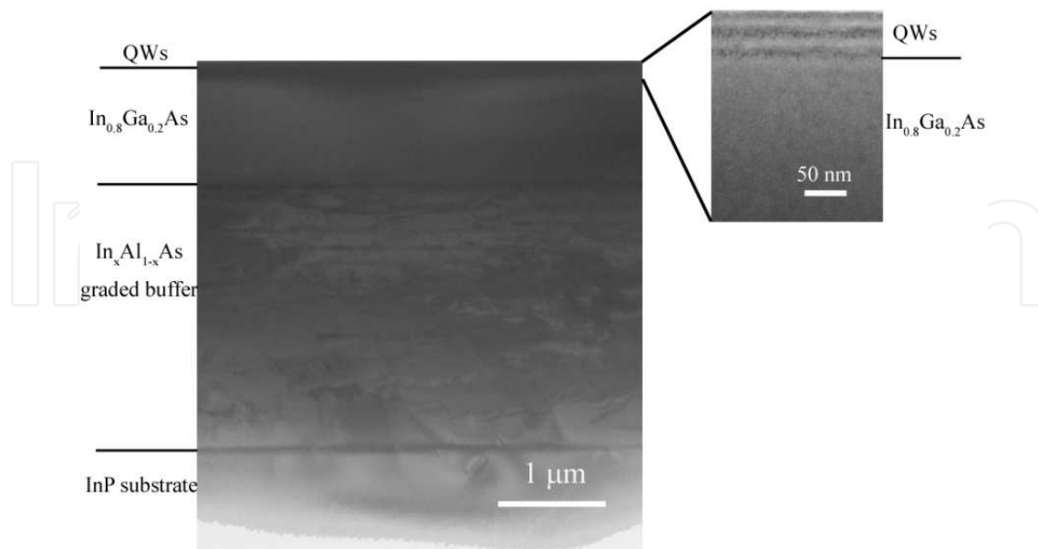
Figure 13. Bright-field XTEM images of the InP-based metamorphic QW epitaxy structure [42]. (Reprinted with permission from AIP)
