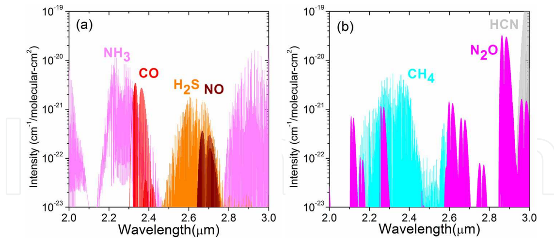
Figure 2. Absorption intensity of (a) \text{NH}_3 , \text{CO} , \text{H}_2\text{S} , \text{NO} molecules and (b) \text{CH}_4 , \text{N}_2\text{O} , \text{HCN} molecules in the 2-3 \mu\text{m} band.
