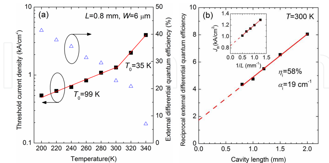
Figure 12. (a) Temperature dependence of the threshold current density and external differential quantum efficiency of the 2.4 \mu\text{m} TQW laser. The lines are the fitting lines of threshold current density in two temperature ranges. (b) Reciprocal external differential quantum efficiency of the TQW lasers as a function of the cavity length at 300 K. The inset shows the threshold current density ( J_{th} ) versus the reciprocal cavity length ( 1/L ). The solid lines are the fitting of the measured data, and the dashed lines are the extrapolated data [38]. (Copyright 2014 The Japan Society of Applied Physics)
