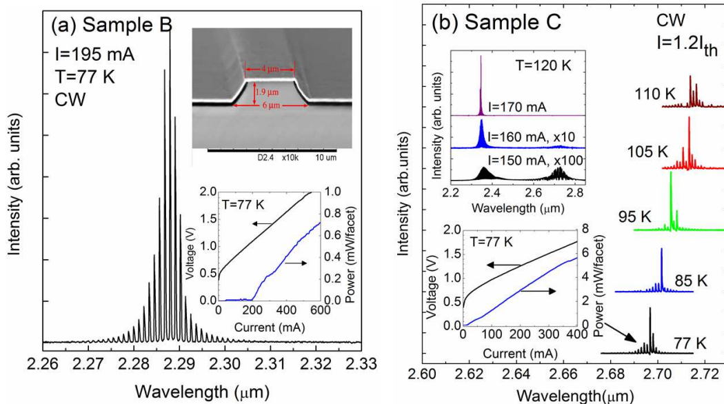
Figure 18. (a) CW lasing spectrum of sample B at 77 K. The upper inset shows the cross-section image of the ridge waveguide structure and the lower inset shows the I-V-P spectra of sample B at 77 K. (b) The temperature-dependent spectra of sample C. The upper inset shows the spectra at different injection currents at 120 K. The lower inset shows the I-V-P spectra at 77 K [55]. (Reprinted with permission from IOP)
