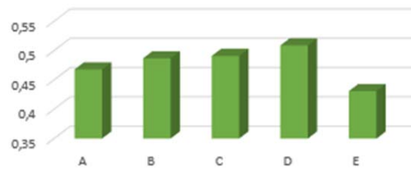
Figure 7. Mean values of PWV at GISM and GANM stations from each strategy (Table 1)
