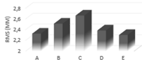
Figure 8. RMS of PWV values at GISM and GANM stations from each strategy (Table 1)
