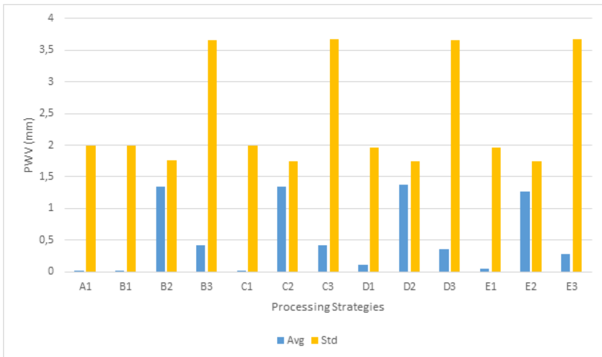
Figure 5. Average and standart deviation of PWV from GANM station for each strategy (Table 1). Values are divided in three time span of 60 day interval since Jan 1st of 2014
