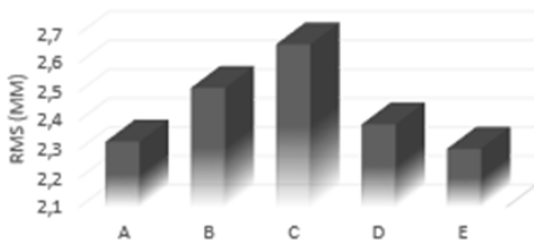
Figure 8. RMS of PWV values at GISM and GANM stations from each strategy (Table 1)
