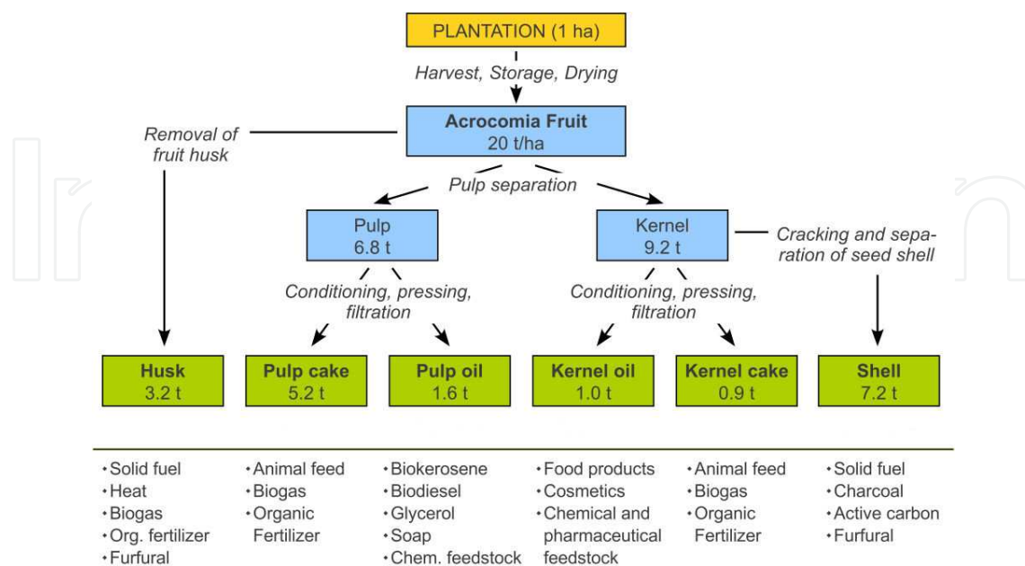
Figure 2. Processing, dry matter yield fractions and uses of macaw palm products [45]
