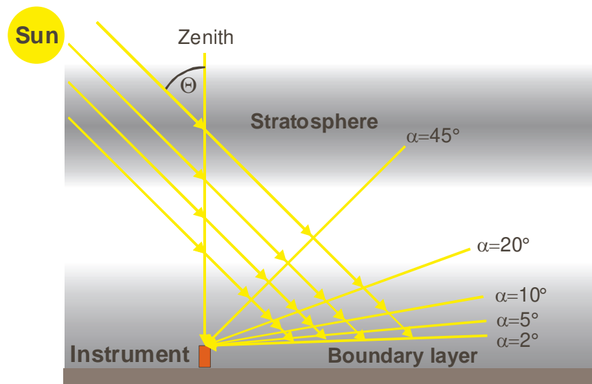
Figure 2. Schematic diagram of MAX-DOAS
