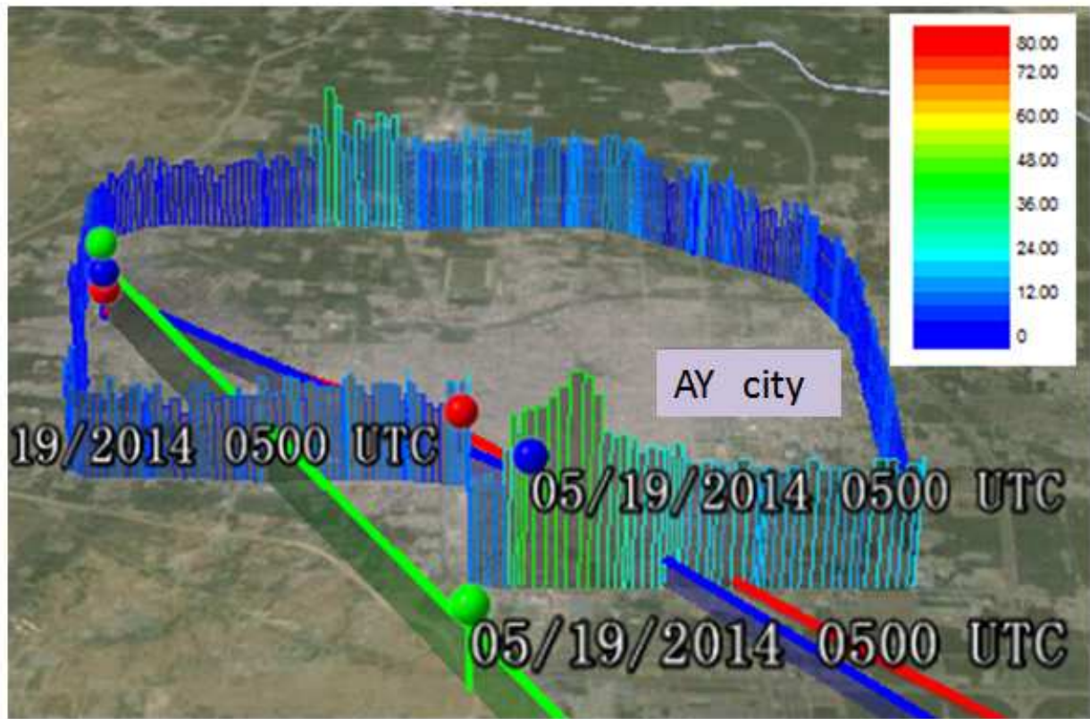
Figure 7. Spatial distribution of \text{SO}_2 and wind field track superposition at AY under northwest wind field
