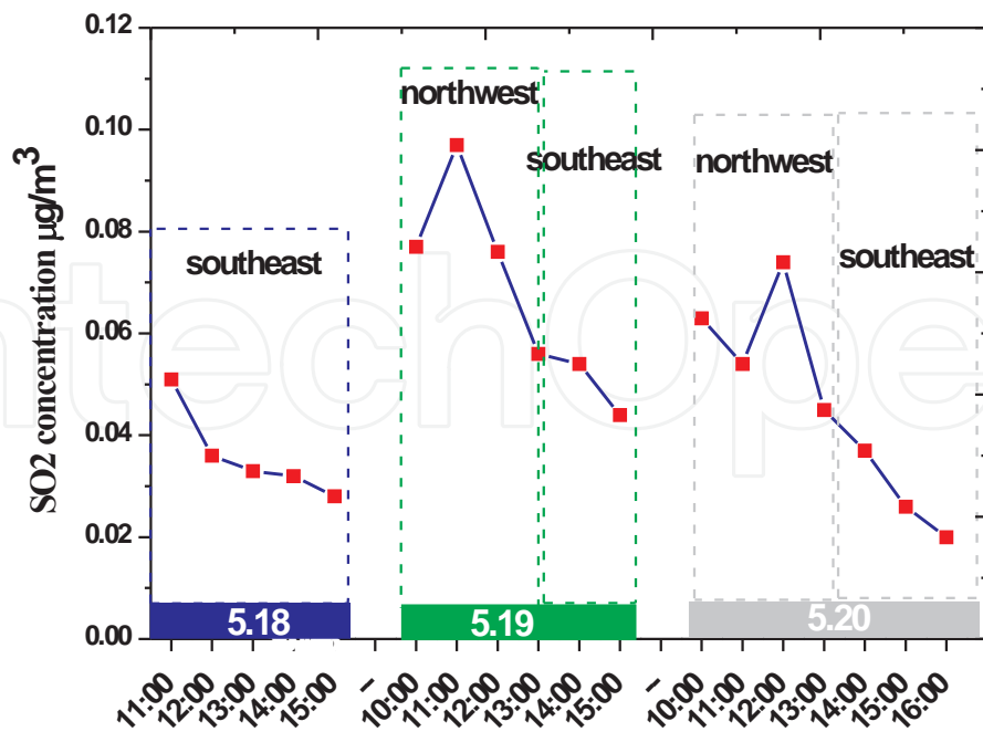
Figure 8. MV/H about ground concentration of \text{SO}_2 in monitoring point at AY
