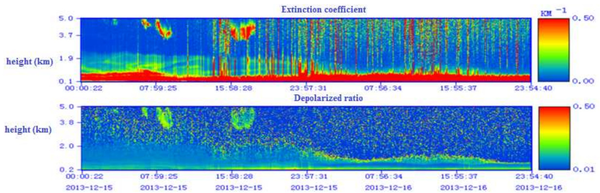
Figure 11. Spatial distributions of aerosols from Dec 15 to Dec 16 at AY, CCR
