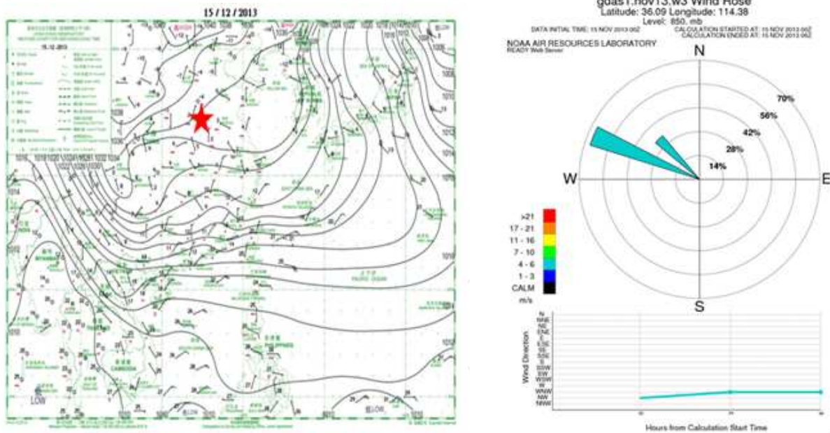
Figure 18. Meteorological conditions and wind rose diagram
