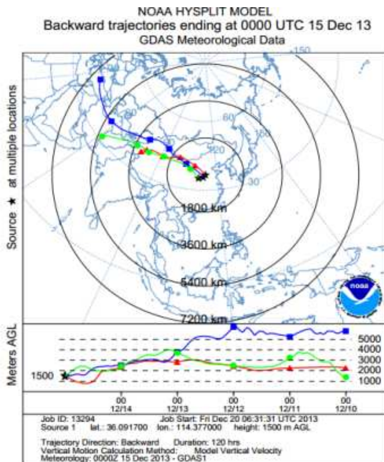
Figure 19. Backward trajectories from Hysplit
