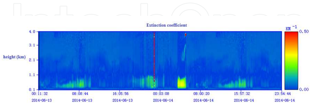
Figure 22. Spatial distribution of aerosol from June 13 to June 14, 2014 at AY, CCR
