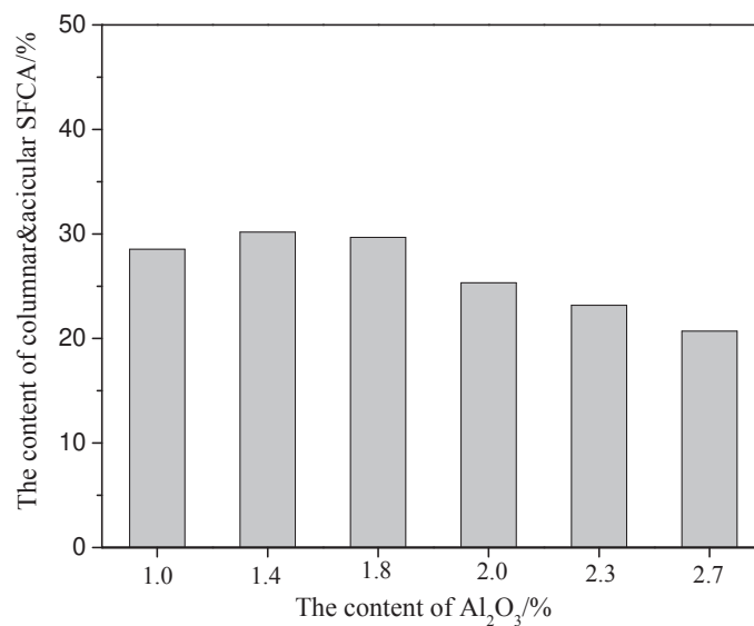
Figure 16. Influence of Al 2 O 3 on the generation of SFCA in melt zone
