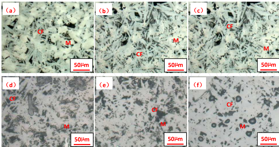
(a) \text{Al}_2\text{O}_3 1.0%; (b) \text{Al}_2\text{O}_3 1.4%; (c) \text{Al}_2\text{O}_3 1.8% (d) \text{Al}_2\text{O}_3 2.0%; (e) \text{Al}_2\text{O}_3 2.2%; (f) \text{Al}_2\text{O}_3 2.6%
