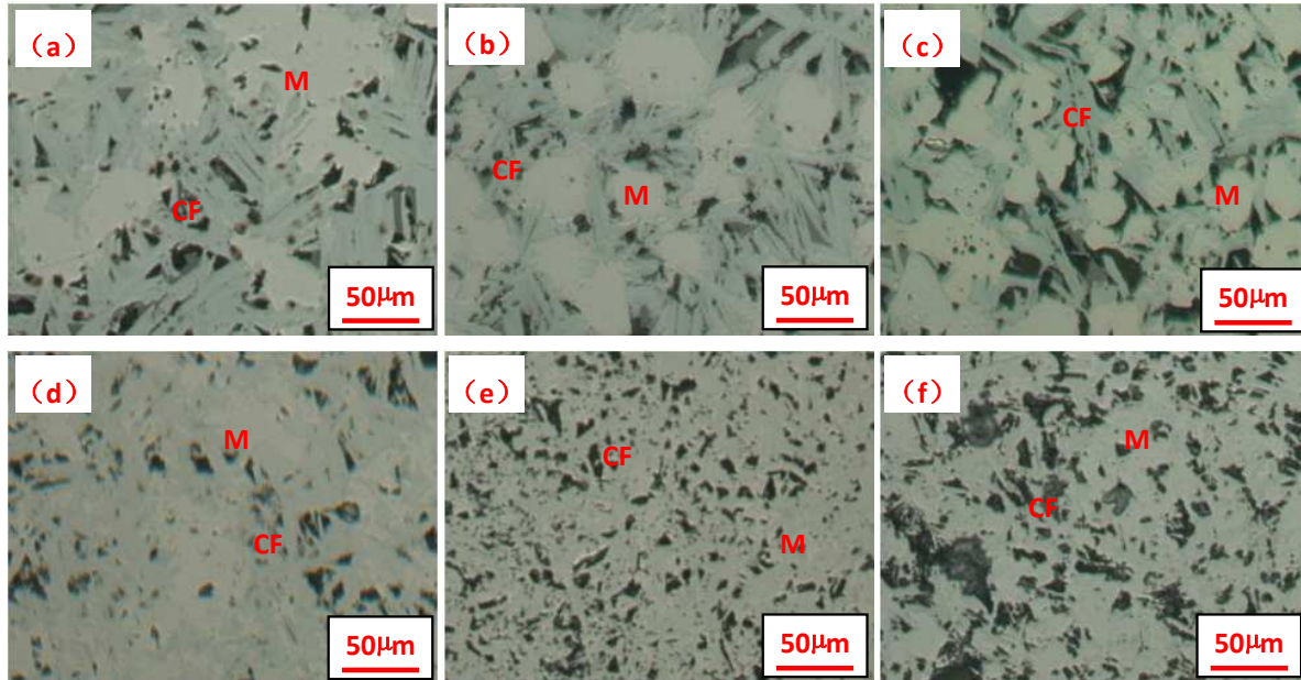
(a) MgO1.4%; (b) MgO2.4%; (c) MgO3.4% (d) MgO4.4%; (e) MgO5.4%; (f) MgO6.4%
