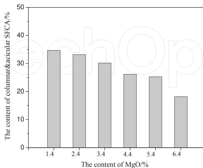
Figure 18. Influence of \text{MgO} on the generation of SFCA in melt zone
