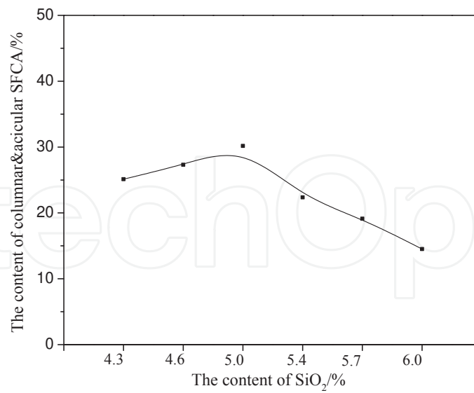
Figure 14. Influence of SiO 2 on the generation of SFCA in melt zone
