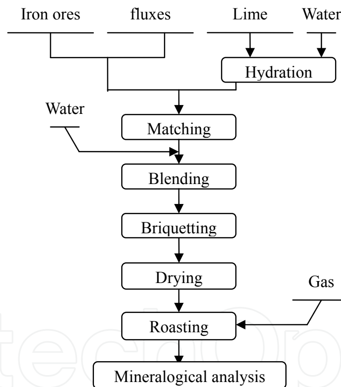
Figure 2. Experimental flow of mini-sintering
