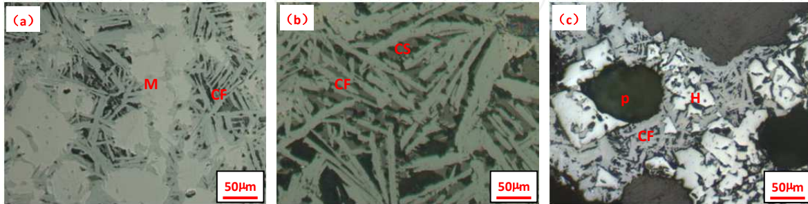
(a) corrosion structure of magnetite and CF, (b) eutectic structure of CF and silicate, (c) pilotaxitic texture of hematite and CF; H—hematite, M—magnetite, CF—calcium ferrite, CS—silicate, P—pole
