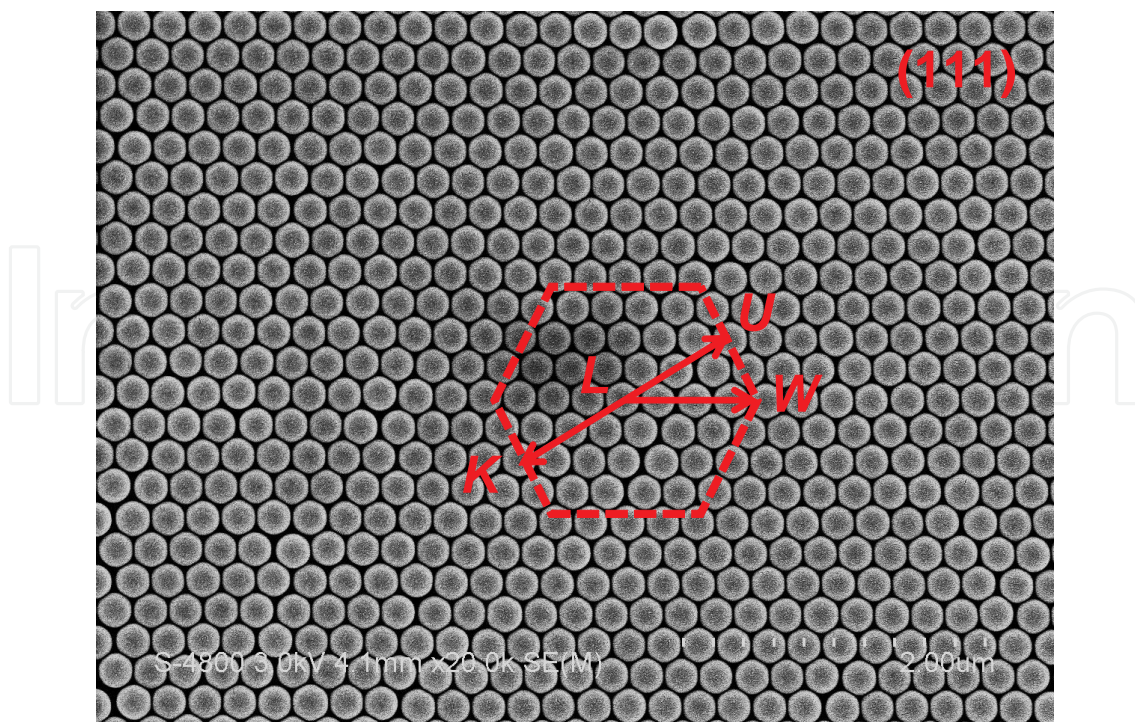
Figure 3. The field-emission scanning electron microscope images of the 3D CPhCs show that the PS nanospheres stack with a well-organized (111) plane. Inset: the first Brillouin zone with the symmetry points.
