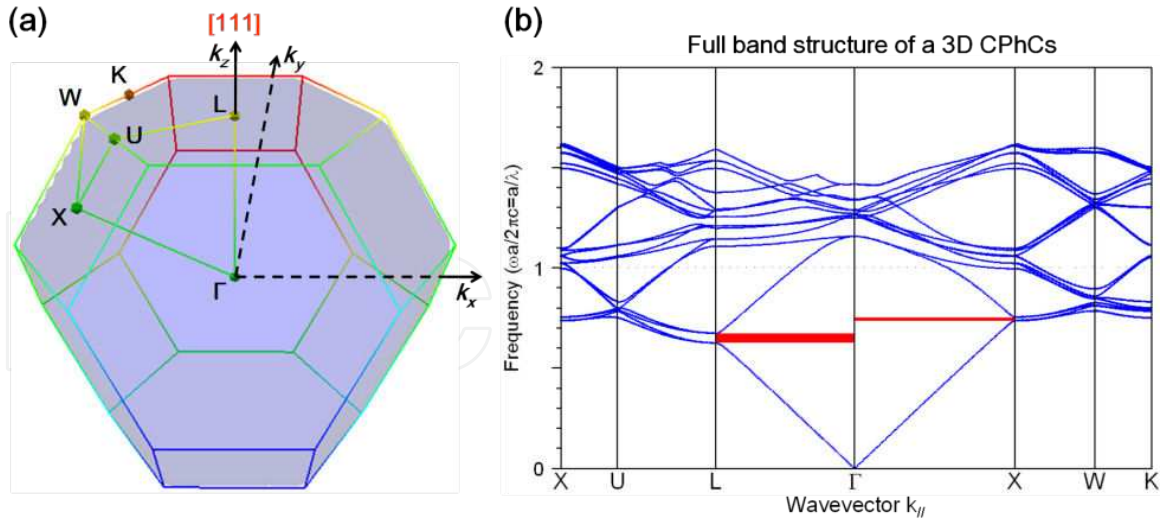
Figure 2. (a) Schematic illustration of the fcc Brillouin zone. (b) The PBS for the lowest-frequency electromagnetic modes of an fcc lattice of close-packed polystyrene (PS) nanospheres ( n_{PS}=1.59 ) in air.
