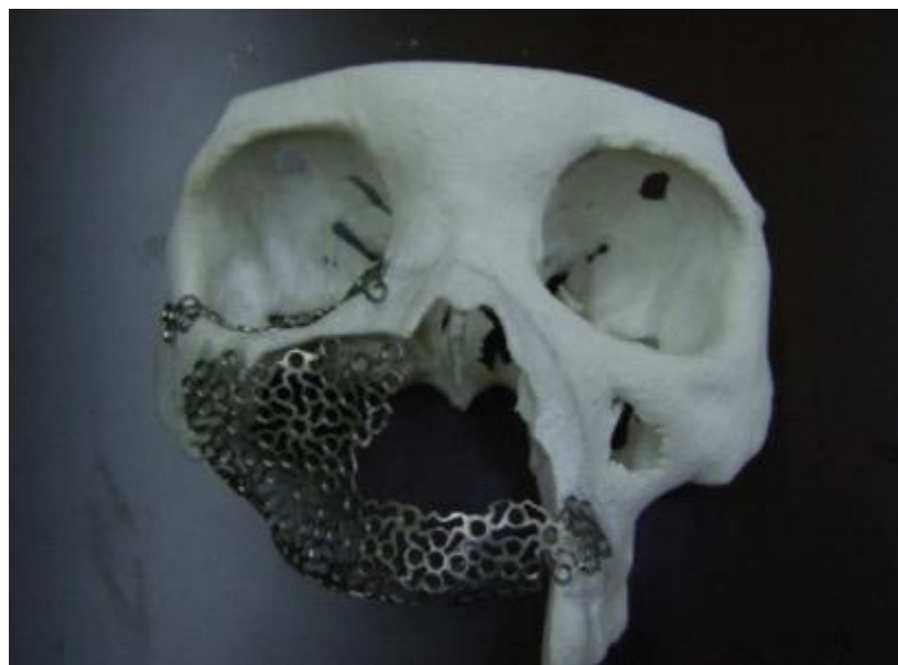
Figure 31. Rapid prototype modelling of maxillofacial prosthesis
