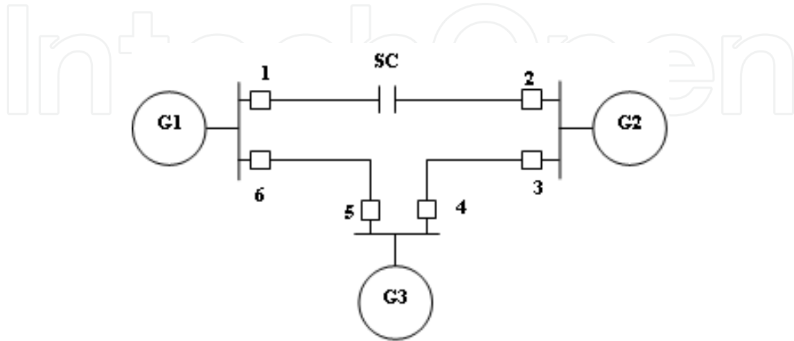
Figure 8. Single line diagram of the 3-bus test system.
