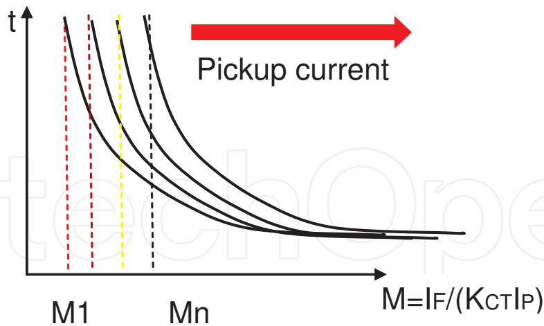
Figure 4. Impact if pickup current value on the relay characteristic curve.
