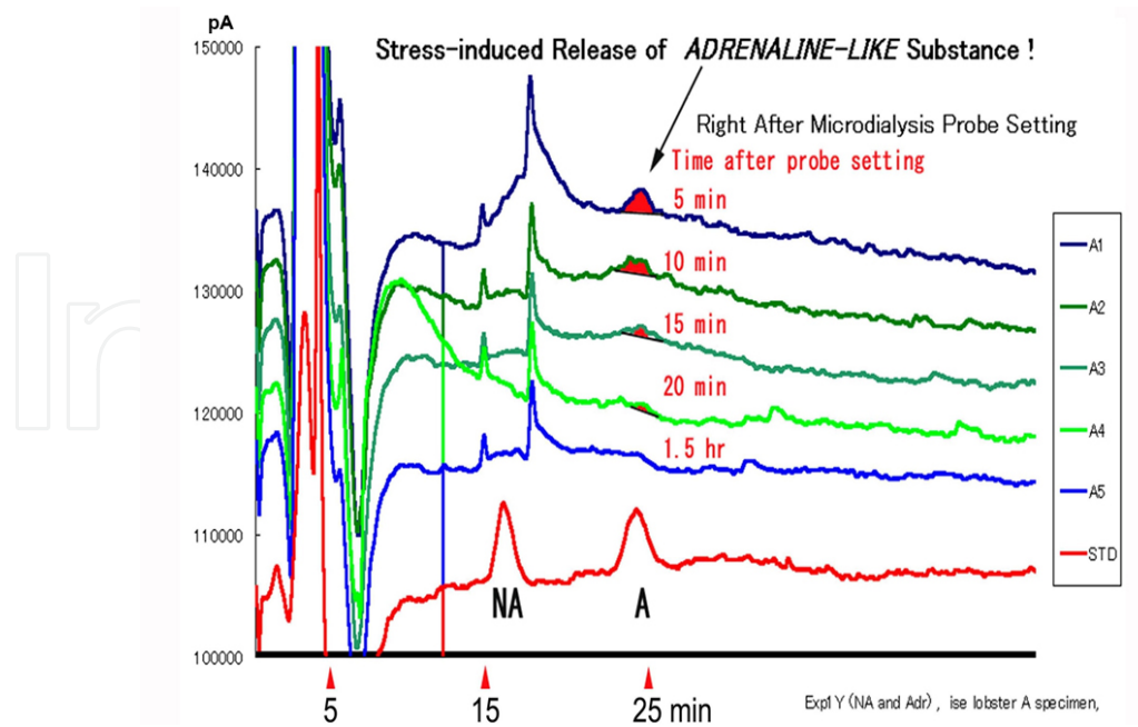
Figure 6. HPLC chart indicating the detection of adrenaline (A) in a Japanese lobster ( Panulirus japonicus ) specimen. Adrenaline release was induced by stress from human handling. Very little adrenaline was detected 20 min and 1.5 hour after the stress stimulus. Therefore, the adrenaline content measured at these times indicates the basal adrenaline content in the blood. Note: noradrenaline (NA) was not detected.
