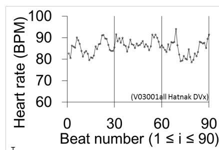
Figure 12. Heartbeat interval time series \{X_i\} and boxes. Ninety beats from 2000 beats are shown.
