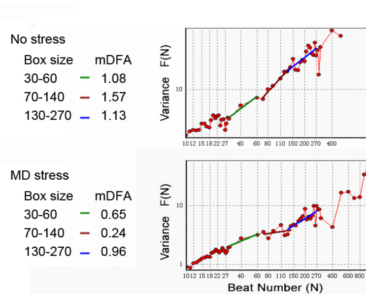
Figure 26. Results of mDFA (program A). Slope and SI for no-stress and MD stress conditions.
