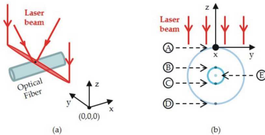
Figure 4. (a) Schematic of coordinates used in this work and (b) optical fiber cross-section indicating the considered referential, the interfaces between the different regions, and points of interest: A – irradiated surface, B – core/cladding interface (upper), C – core/cladding interface (lower), D – bottom surface and E – middle point. The origin of the reference system is in the middle of the laser line.
