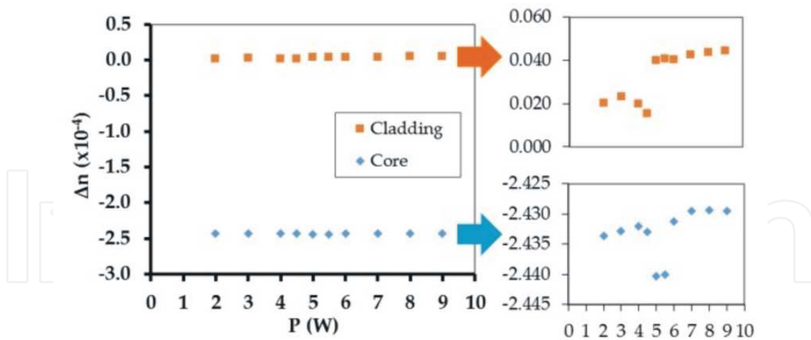
Figure 15. Calculated (maximum) refractive index change at the core and cladding for different applied laser powers. ( t_{on}=0.6 s; F=0.461 N).
