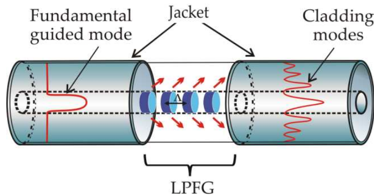
Figure 1. Schematic diagram of a mode coupling in a long period grating [11].
