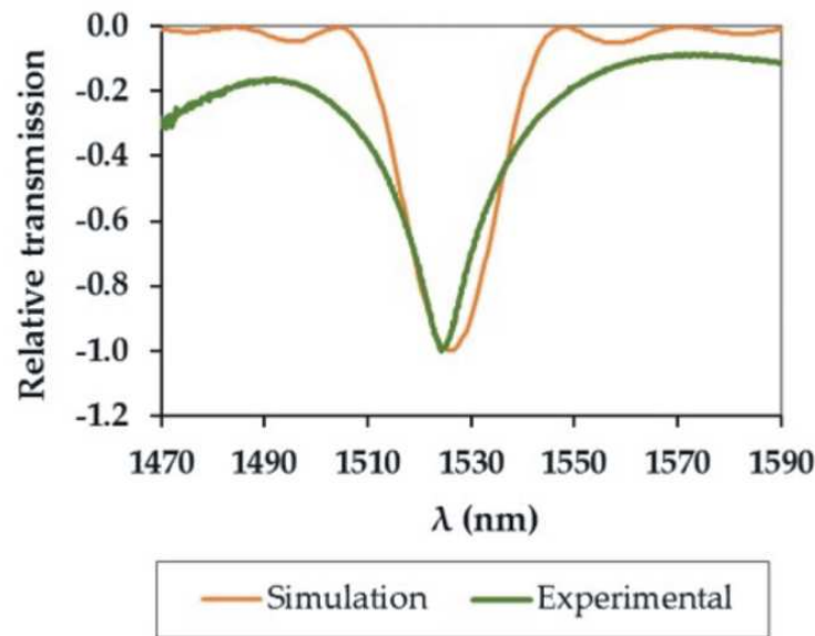
Figure 18. Experimentally obtained and simulated relative normalized spectral transmission under the same conditions considered in Figure 17.
