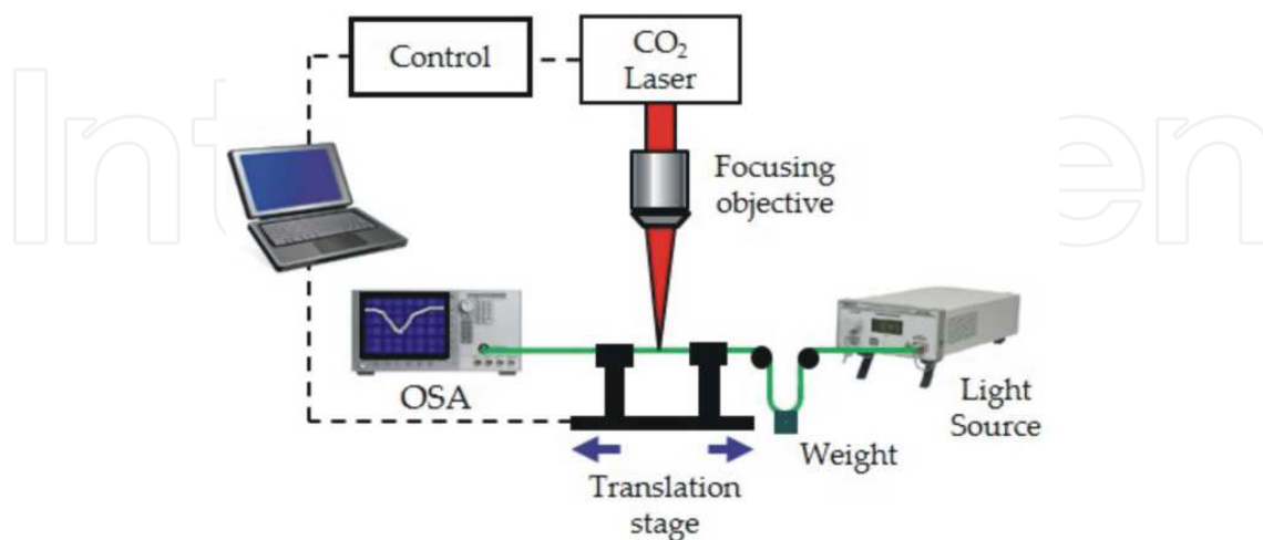
Figure 3. Schematic diagram of a typical LPFG fabrication system based on the point-to-point technique using a CO 2 laser.
