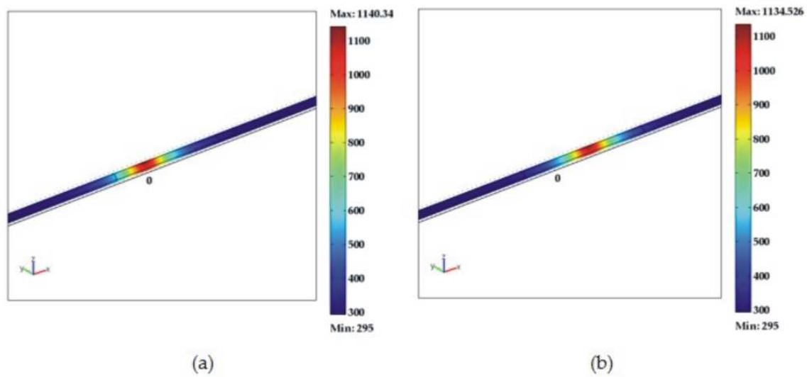
Figure 9. Temperature distribution in the implemented 3D geometry for the laser irradiation of an optical fiber ( P=6 W; t_{on}=0.6 s; F=0.461 N; \Delta t=1 s; \Delta x=500 \mu\text{m} ), at (a) t=0.6 s and (b) t=2.2 s. Colour bar values are in K.
