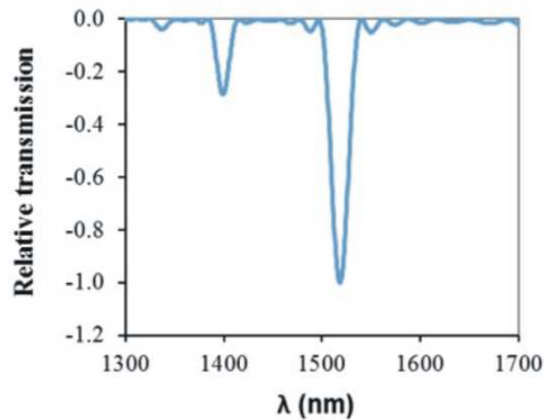
Figure 2. Theoretical example of the spectrum of a 500 \mu\text{m} -LPFG inscribed in a Corning SMF-28 fiber.
