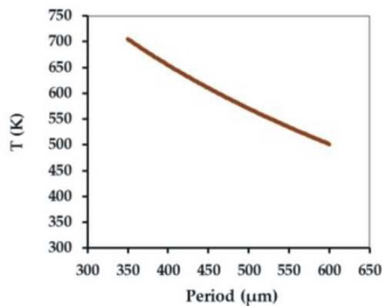
Figure 11. Maximum temperature at x=0 m when the laser is irradiating at x=\Delta x for different values of \Delta x (LPFG period). ( P=6 W; t_{on}=0.6 s; \Delta t=1 s; F=0.461 N).
