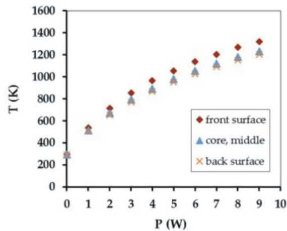
Figure 14. Maximum temperature calculated for different laser powers, at x=0 m. ( P=6 W; t_{on}=0.6 s; F=0.461 N).
