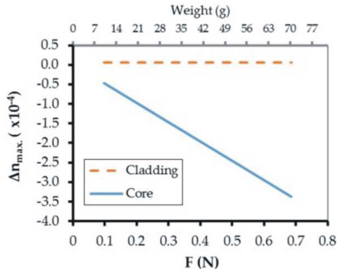
Figure 16. Calculated refractive index change (maximum change for core and cladding) for different applied draw tensions. ( P=6 W; t_{on}=0.6 s; F=0.461 N).
