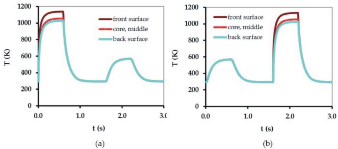
Figure 10. Plots of the temperature evolution during laser irradiation and cooling at (a) x=0 m and (b) x=\Delta x . ( P=6 W; t_{on}=0.6 s; F=0.461 N; \Delta t=1 s; \Delta x=500 \mu\text{m} ).
