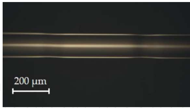
Figure 17. Picture showing two irradiated zones from a 25 mm LPFG with 500 \mu\text{m} period written on a SMF-28 optical fiber. ( P \approx 6 \text{ W} ; t_{\text{on}}=0.6 \text{ s} ; \Delta t=1 \text{ s} ; F \approx 0.5 \text{ N} )
