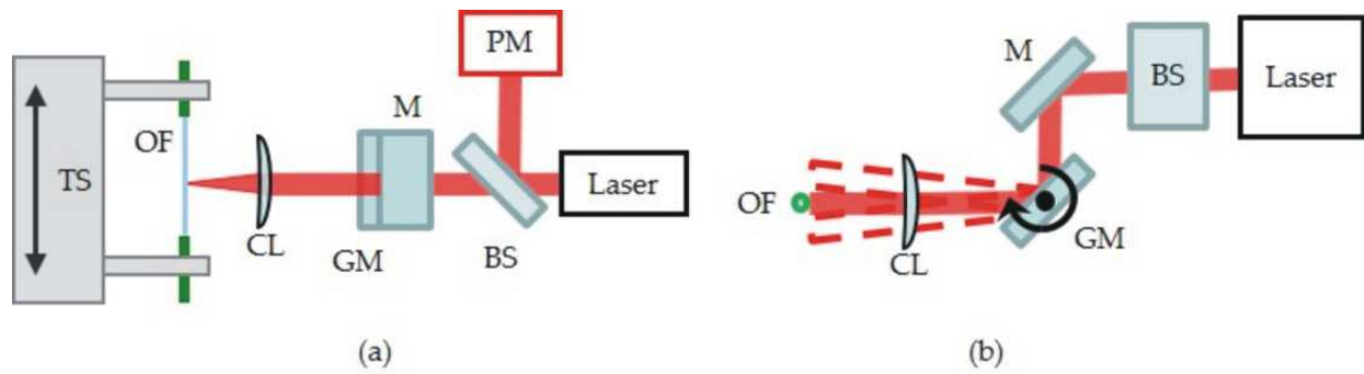
Figure 7. (a) Top and (b) lateral schematic views of the optical setup. BS – beam splitter; CL – cylindrical lens; GM – galvanometric mirror; M – mirror; OF – optical fiber; PM – power meter; TS – translation stage.
