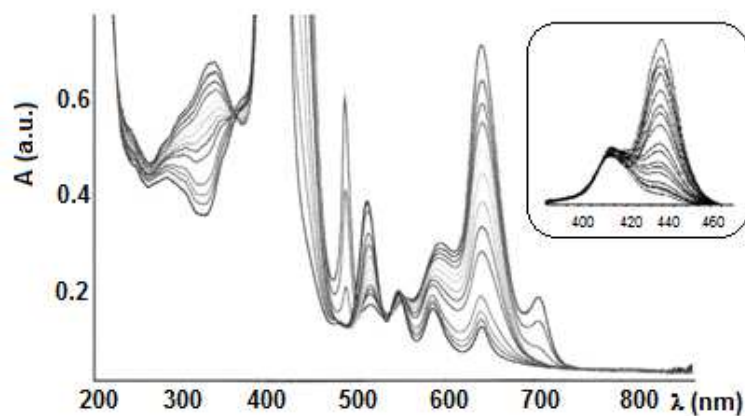
Figure 15. The aggregation equilibrium of TPPS 4
