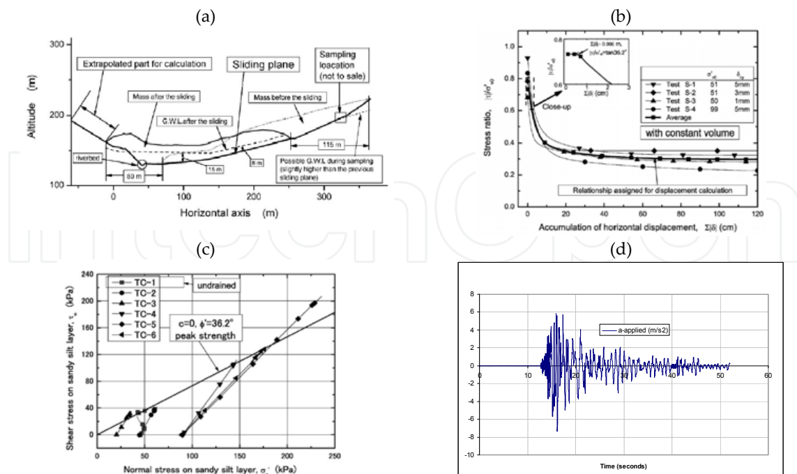
Figure 6. The Higashi Takezawa landslide. (a). Cross-section of slide (Deng et al. [1]), (b). Simple shear test results (Deng et al. [1]), (c) Triaxial test results (Deng et al. [1]), (d) representative applied acceleration in terms of time (Deng et al. [1])
