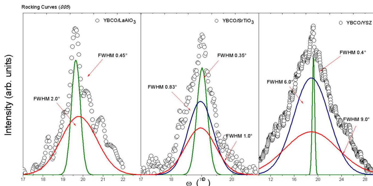
Figure 8. Rocking curves corresponding to the (005) reflection of the YBCO films obtained by CSD on \text{LaAlO}_3 , \text{SrTiO}_3 and YSZ substrates, after oxygenation at 860^\circ\text{C} . The rocking curves corresponding to the sample deposited on \text{LaAlO}_3 can be fitted with two Gaussian functions, while the samples deposited on \text{SrTiO}_3 and YSZ can be fitted up to three Gaussian functions respectively. Each Gaussian function provides a different \Delta\omega value which is listed in Table 4.
