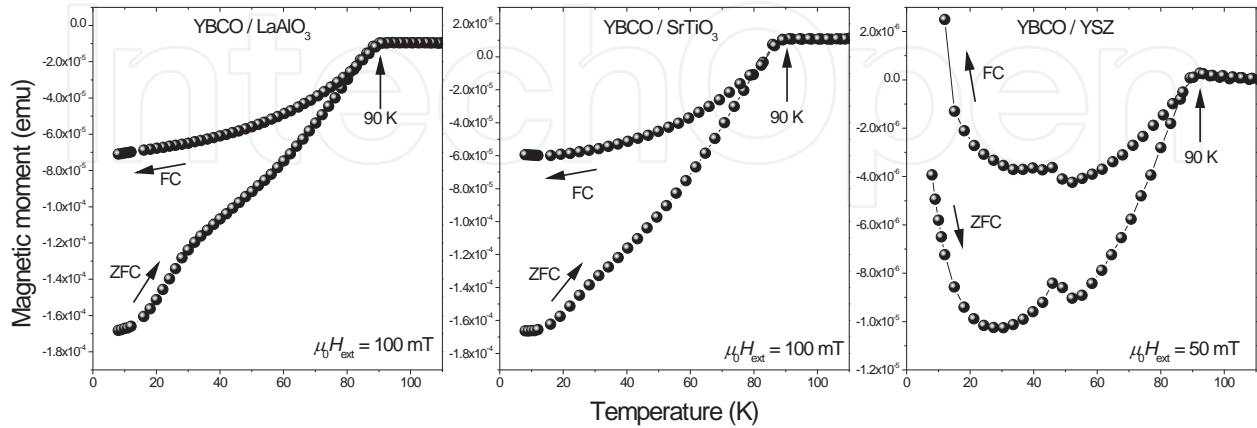
Figure 9. Magnetic moment vs. temperature of YBCO films on \text{LaAlO}_3 , \text{SrTiO}_3 and YSZ substrates obtained by oxalate CSD and oxygenation at 860 °C. The magnetic measurements were taken in zero field cooling (ZFC) and field cooling (FC) modes. The superconducting property is demonstrated by the diamagnetic signals below the transition temperature 90 K. The samples deposited on \text{LaAlO}_3 and \text{SrTiO}_3 were measured under \mu_0 H_{ext}=100 mT while the sample deposited on YSZ was measured under \mu_0 H_{ext}=50 mT.
