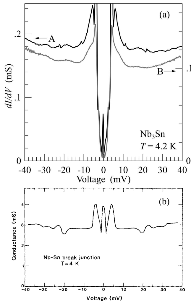
Figure 4. (a) G(V) describing different Nb_3Sn break junctions. (b) The break-junction data of the superconducting Nb-Sn composite (taken from Ref. [30]).
