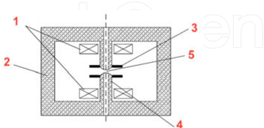
Figure 11. Sketch of prospective setup for a TEM objective lens [20]. Coils (1) provide magnetic flux through the yoke (2). Two stabilizing SC rings (3) are placed near the pole piece ends (4) to stabilize magnetic field in the sample area (5).
