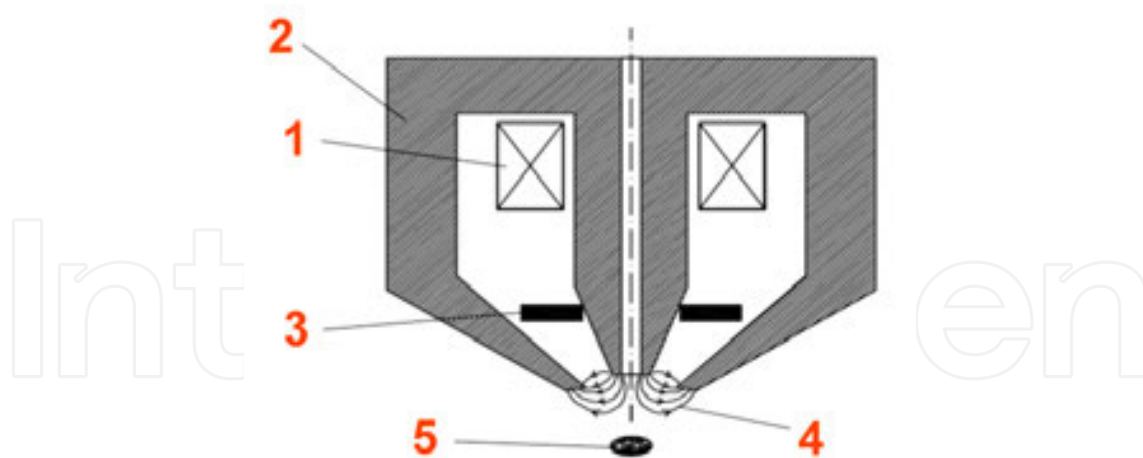
Figure 14. Sketch of prospective setup for an SEM conical objective lens [20]. Coil (1) provides magnetic flux through a yoke (2). A stabilizing SC ring (3) is placed near the pole piece end to stabilize the magnetic field in the area of the strong magnetic field gradient (4), which focuses the electron beam onto the sample.
