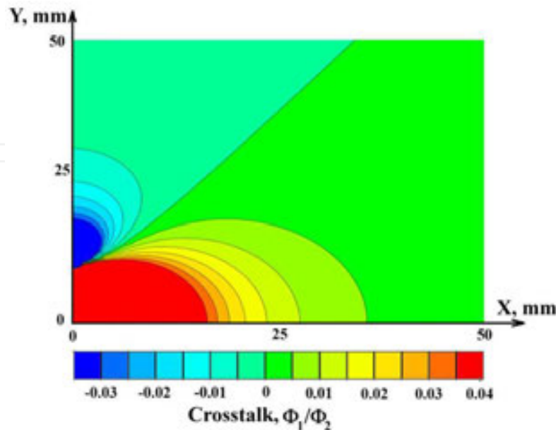
Figure 20. Crosstalk calculation according to Eqs. (4) and (5).
