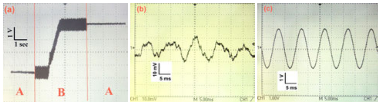
Figure 9. (a) Oscillogram showing measured magnetic field in stabilized (A) and adjusted (B) modes in the test setup. In the additional interference, which was simulated by adding an AC field to the main (DC) field of the coil, appeared as a change of a different value during heating of the superconducting ring. (b) Test signals with SC stabilizer ON and (c) with SC stabilizer OFF.
