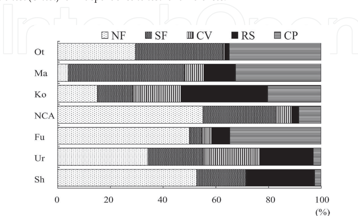
Figure 4. Compositions of vegetation types (NF: natural forest; SF: secondary forest; CV: coastal vegetation; RS: rice fields and swamps; CP: croplands and pastures) within the home ranges of the Iriomote cat in seven study sites (Ot: Otomi; Ma: Maira; Ko: Komi; NCA: northern coastal area; Fu: Funaura; Ur: Urauchi; Sh: Shirahama).
