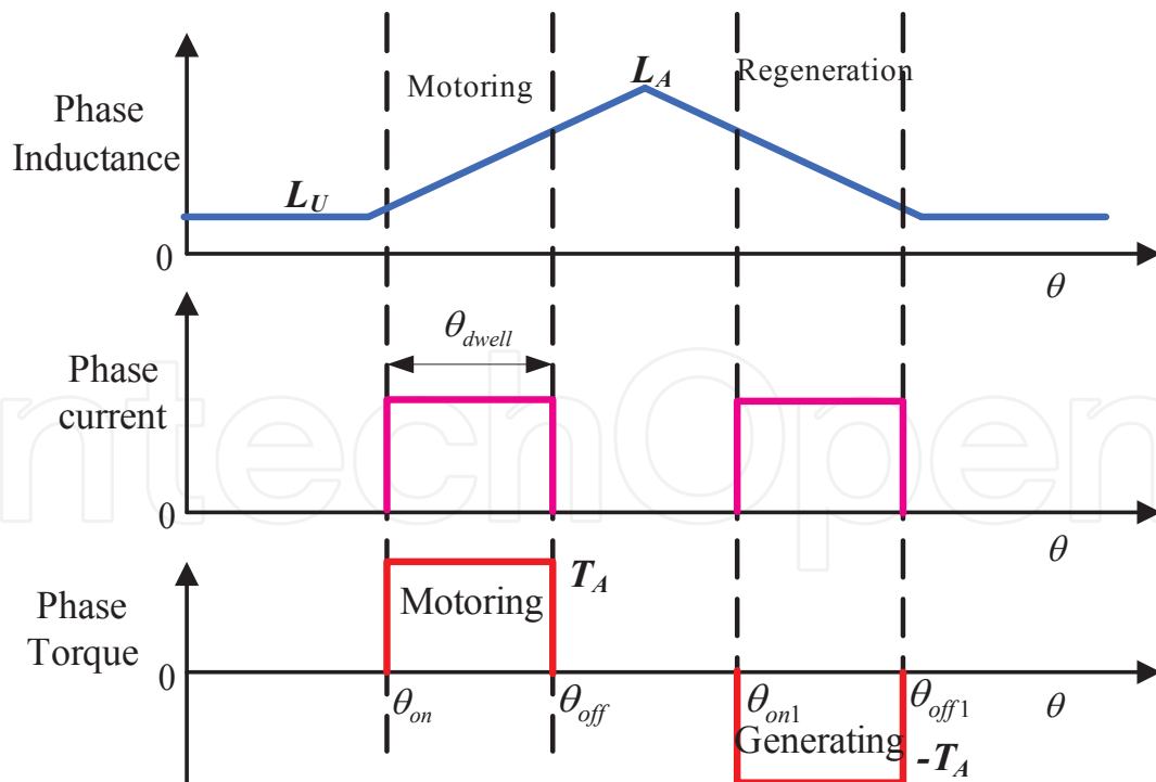
Figure 3. Motoring and regeneration modes of SRM
