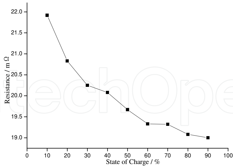
Figure 17. Resistance as a function of SOC
