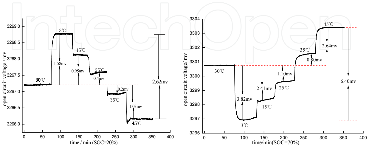
Figure 15. OCV under different temperature (the first and the second subplots respectively correspond to the cases in which SOC=20% and SOC=70%)
