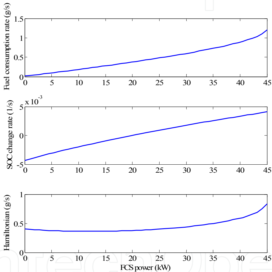
Figure 26. An example of solving the optimal FCS net power according to the PMP
