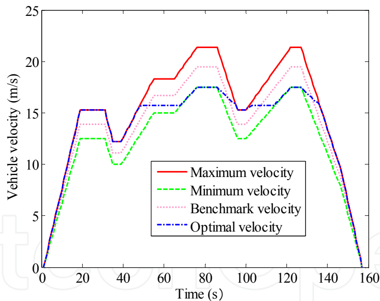
Figure 28. The optimal vehicle velocity profile and the benchmark velocity profile
