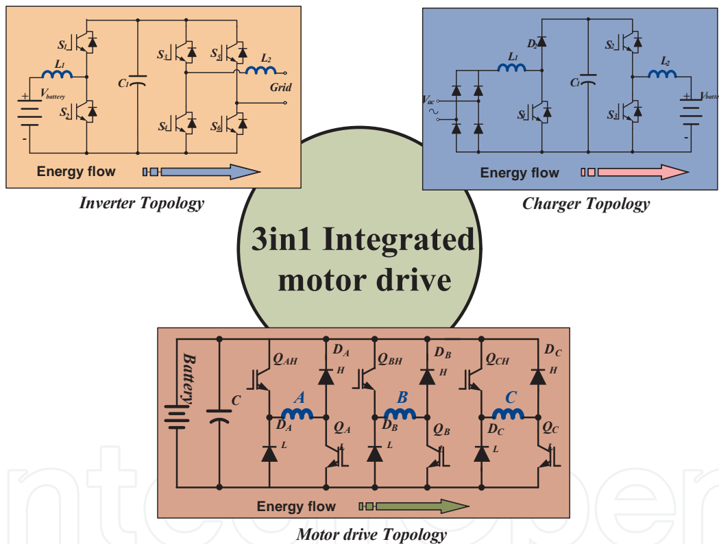
Figure 6. The circuit topology of motor drive, charger, and inverter
