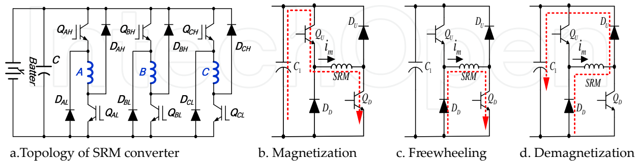
Figure 4. Conventional 3-phase SRM drive and its operation modes
