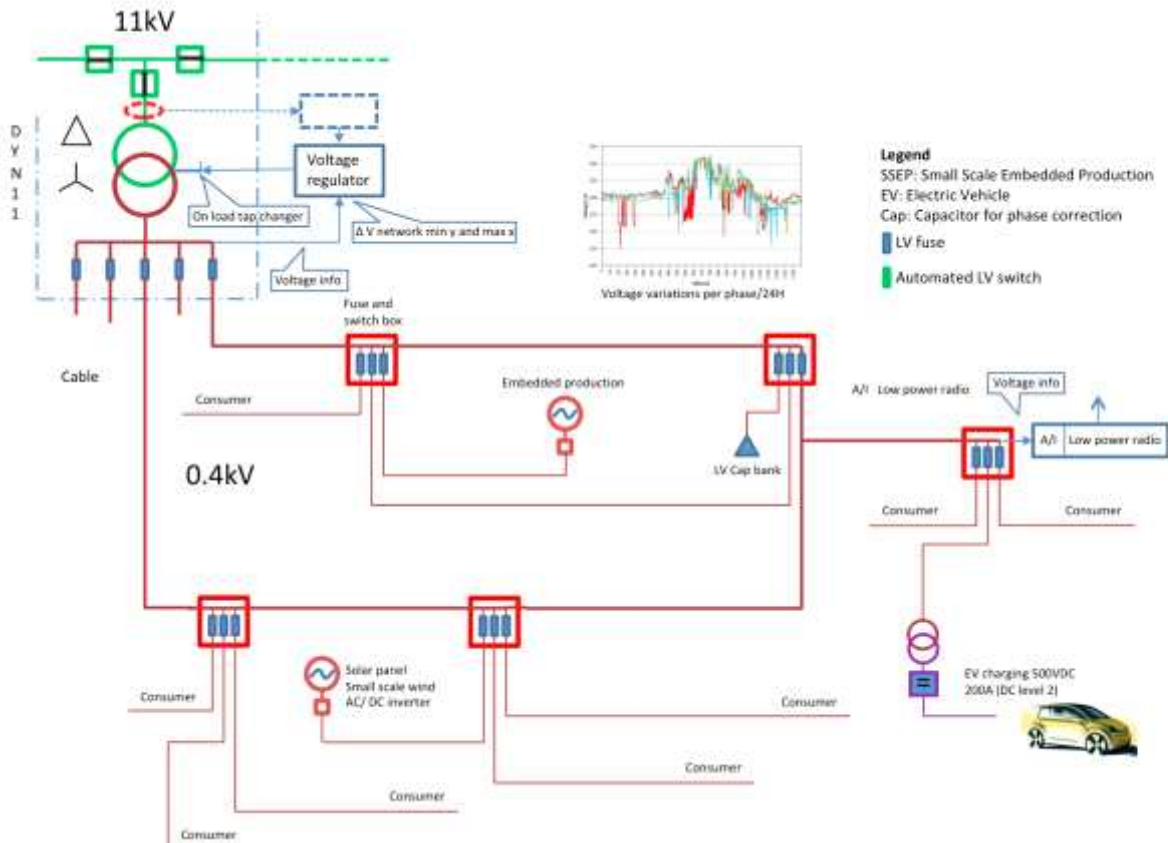
Figure 13. Smart equipment supporting cutting losses in distribution grids
