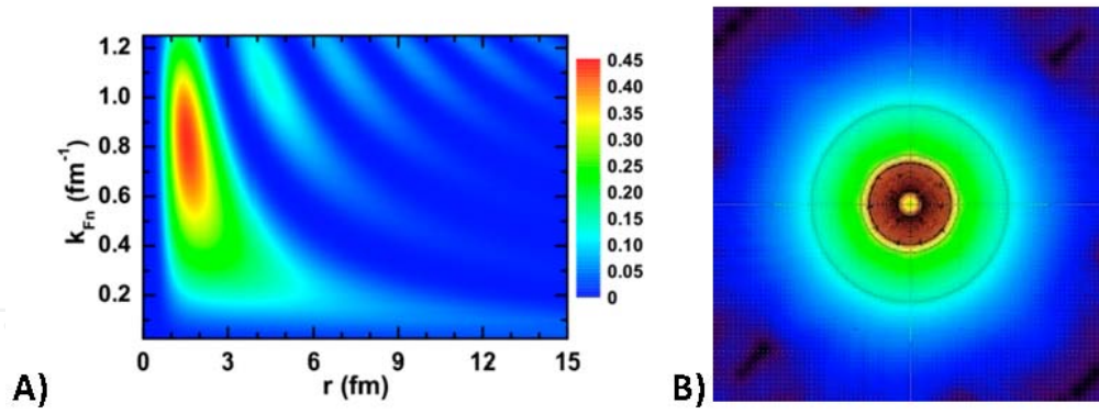
Figure 8. A). Fermionic distribution of probability density r^2|\Psi_{\text{pair}}(r)|^2 of the neutron Cooper pairs as a function of the neutron Fermi momentum kF_n and the relative distance r between the pair partners in symmetric nuclear matter [22]. This can produces Eddy currents with the property anti-gravitational current given in (83). B). The part colored in blue determines the absence of magnetic flow, such like is wanted that it happens for the super-currents existence on the surface of a levitating vehicle, making that this everything behaves as a diamagnetic, except in the central ring colored in red and yellow where exists an intense magnetic field ( this simulation was published in the Proceedings of Fluid Flow, Heat Transfer and Thermal Systems of ASME in the paper IMECE2010-37107, British Columbia, Canada with all rights reserved © [9]).
