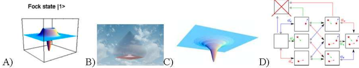
Figure 9. A) The quasi-particle region: holes. The fermionic Fock superconducting space for one particle: observe the two phases of fermion spaces, upper surface corresponds to the holes zone. Of fact this zone is like volcano, since in their interior are holes. The below surface is the free fermions whose behavior is seemed to the Bose-Einstein distribution. B). Structure of the ship transmitting the change phase of the particles that come from of the ship reactor [29, 30]. C) Electro-twistor generated by the magnetic field-superconducting interaction [9]. D) Appearing of the creation operators that shape the wrapping space over structure of the ship. This is defined by a fermionic Fock space, for example under the ship as the impeller twistor [23].
