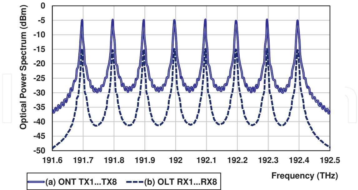
Figure 11. Optical power spectra of transmitted signals for laser based WDM-PON upstream direction: (a) on the output of ONT transmitters and (b) on the input of OLT receivers after 20 km transmission.
