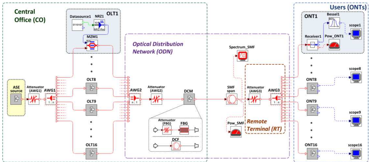
Figure 6. Simulation model of proposed high-speed up to 16-channel AWG filtered and ASE seeded SS-WDM PON system with DCM module.
