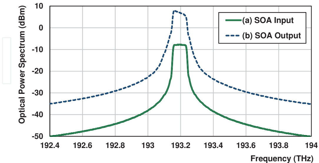
Figure 9. Optical spectra of spectral slices filtered by AWG1 demultiplexer: (a) before SOA and (b) on the output of SOA after amplification.
