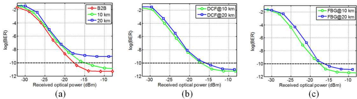
Figure 18. BER versus received optical power at the receiver for 8-channel SS-WDM PON system (a) without CD compensation, (b) using DCF for CD compensation, (c) using FBG for CD compensation.
