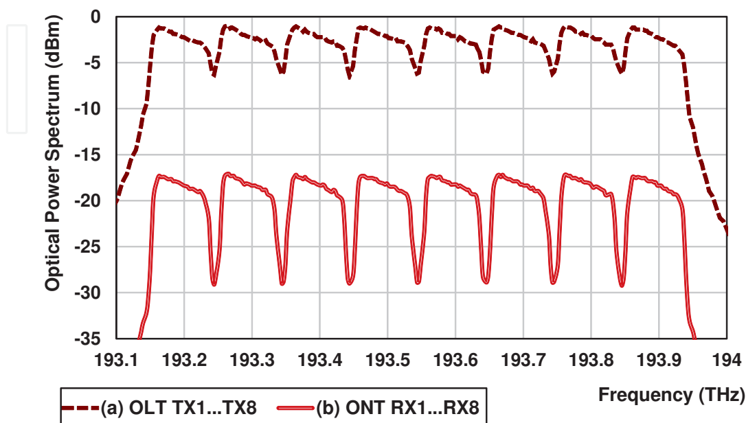
Figure 10. Optical power spectra of transmitted signals for spectrum-sliced WDM-PON downstream direction: (a) on the output of OLT transmitters and (b) on the input of ONT receivers (users) after 20 km transmission.
