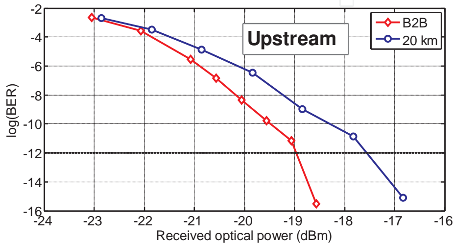
Figure 15. Measured BER performance of separate laser based upstream light signals in B2B configuration and after transmission through 20 km SMF fiber span.
