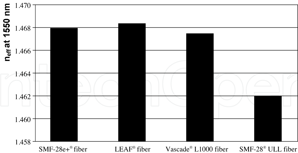
Figure 1. Effective group index of refraction impact of various commercially available Corning single mode fiber types [28].
