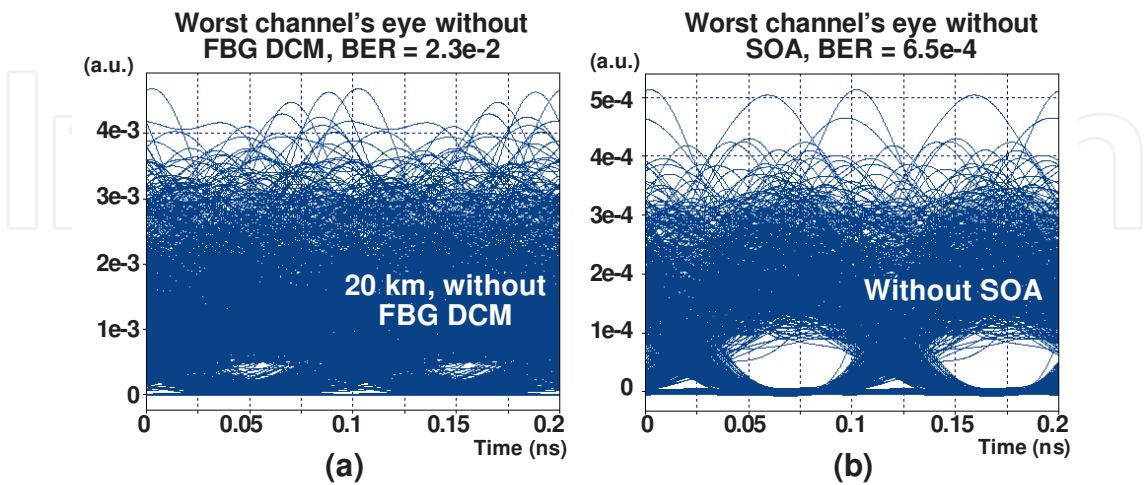
Figure 12. Received eye diagrams of downstream signals for bidirectional 8-channel spectrum sliced WDM-PON system: (a) after 20 km without FBG DCM for CD compensation and (b) without use of SOA for noise suppression (B2B measurement).
