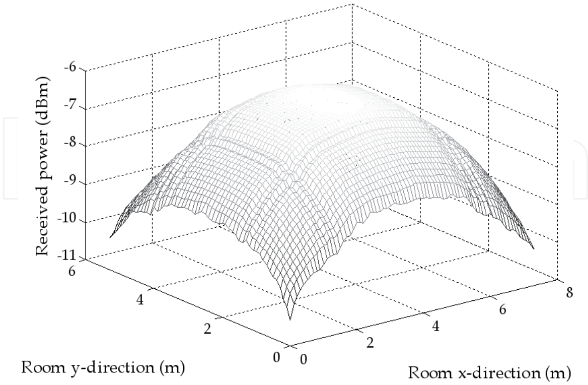
Figure 10. Power balance at the receiver plane for the imaging receiver ( P_{min}=-10.4 dBm; P_{max}=-6.2 dBm; \bar{P}=-7.4 dBm).
