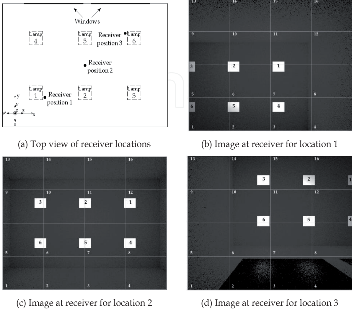
Figure 7. Images impressed on photodetector surface for three different receiver locations.
