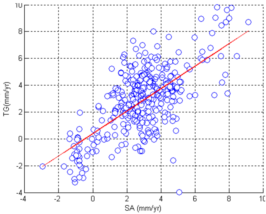
Figure 7. Correlation coefficients between SA and TG trends
