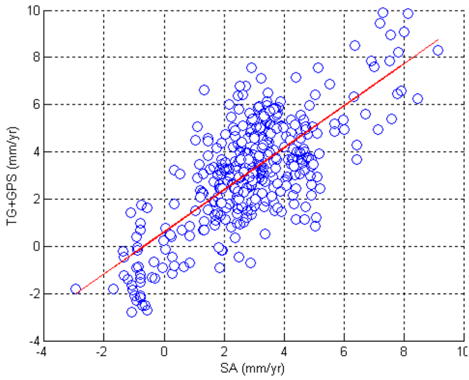
Figure 6. Correlation coefficients between SA and TG+GPS trends
