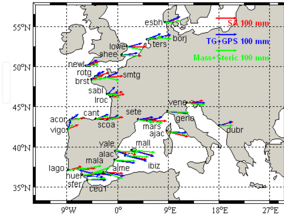
Figure 9. Annual amplitudes and annual phases of sea level changes along the Southwest European coasts at 31 TG stations (TG + GPS (blue), Satellite altimetry (red), GRACE Mass + Steric results (green)). The arrow lengths show the amplitudes and the phases expressed by Eq (3) are counted as clockwise from the north.
