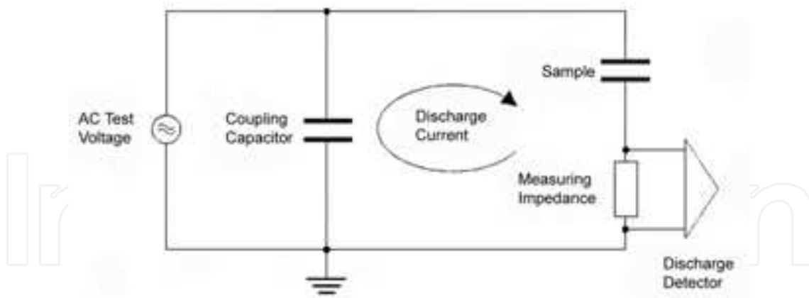
Figure 3. Discharge detection circuit.
