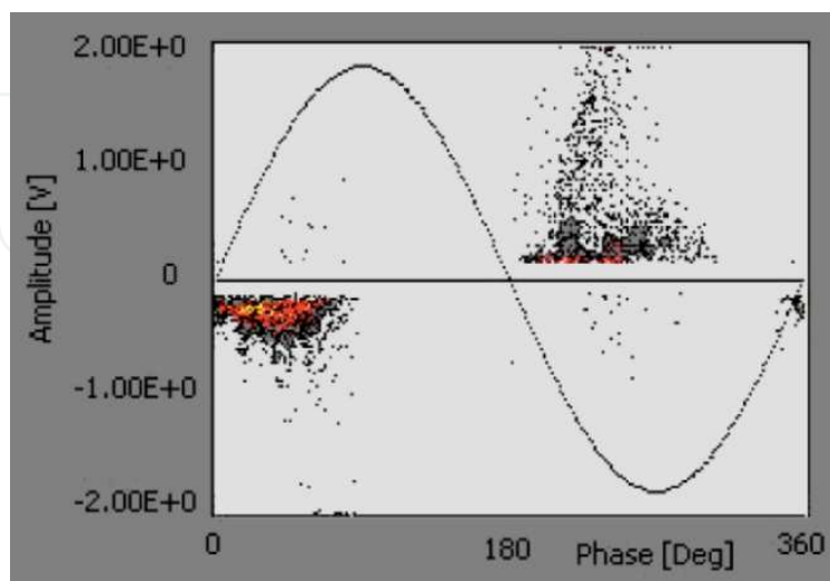
Figure 8. PD Pattern of surface discharges.
