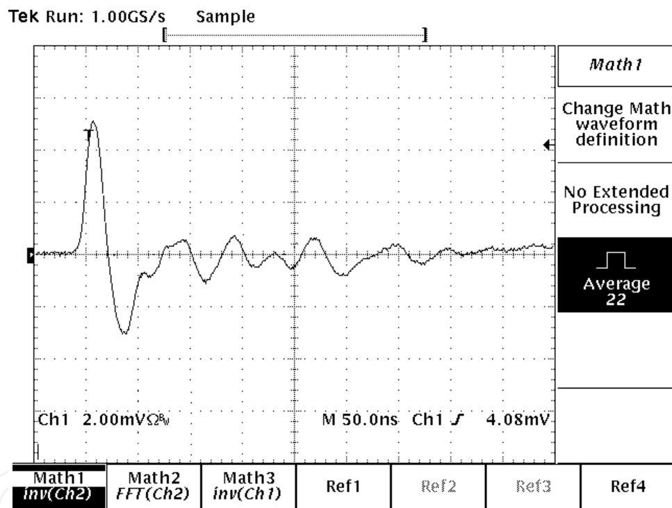
Figure 4. Generic second order PD Pulse.
