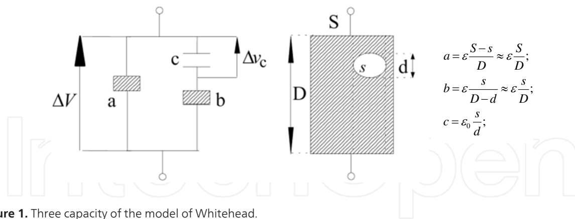
Figure 1. Three capacity of the model of Whitehead.
