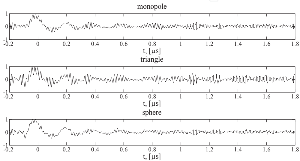
Figure 21. Time profiles of the received voltage.
