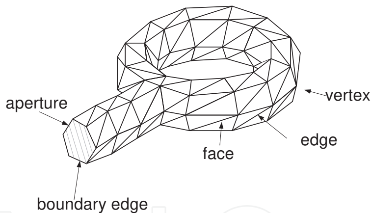
Figure 10. Loop antenna described with triangular surfaces
