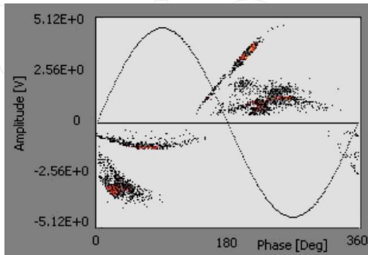
Figure 7. PD Pattern of internal discharges.
