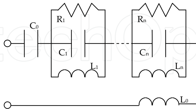
Figure 24. Foster's canonical form for an electrical antenna.
