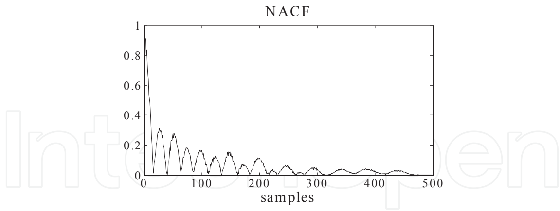
Figure 22. NACF of the PD current of Figure17.
