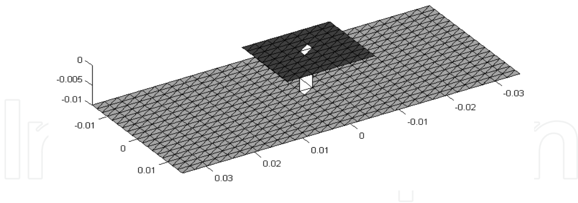
Figure 16. Discrete surface MoM model of the emitting source.
