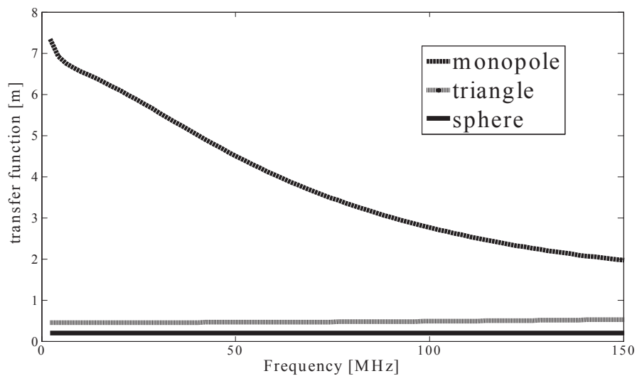
Figure 20. Transfer function of the three antennas for the range of 0-150MHz.
