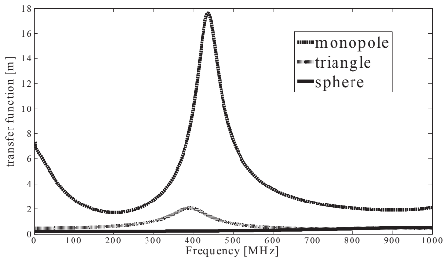
Figure 19. Transfer function of the three antennas.
