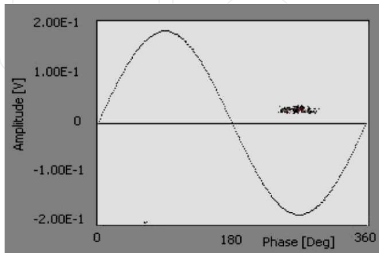
Figure 9. PD Pattern of corona discharges.
