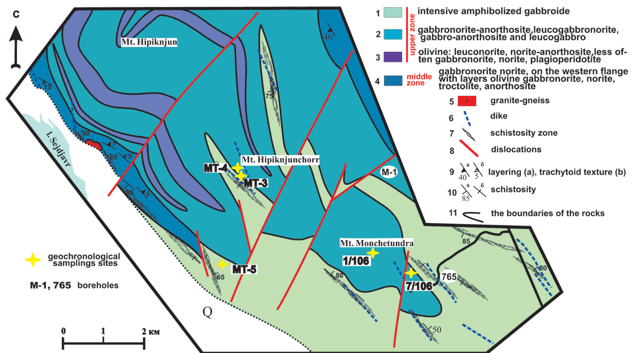
Figure 7. Schematic geological map of the central and southeastern parts of the Monchetundra intrusion (compiled by L.I. Nerovich on the materials of Central Kola Expedition OAO, Geological Institute KSC RAS with additions and amendments).
