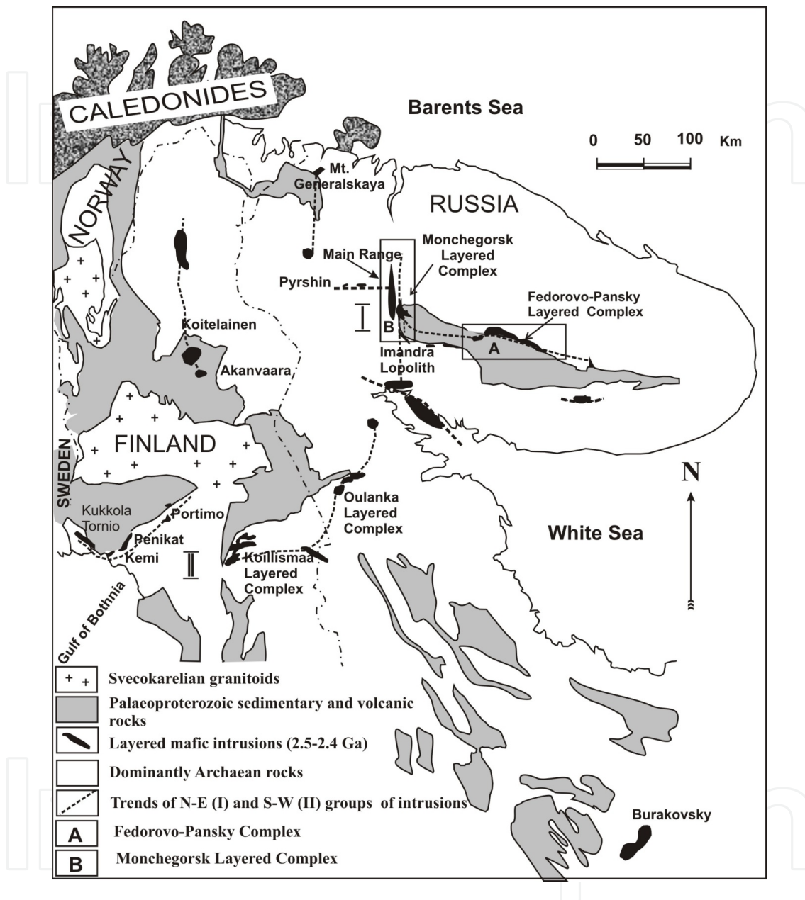
Figure 1. Generalized geological map of the northeastern part of the Baltic Shield and the location of Paleoproterozoic mafic layered intrusions (Mitrofanov et al., 2005).
