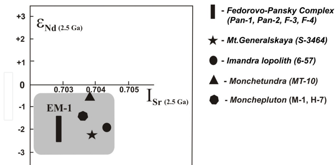
Figure 11. Isotope \epsilon_{Nd}, I_{Sr} plot of rocks from the Northern (Kola) Belt layered intrusions. Grey colour in the diagram shows EM-1 reservoir plotted for the layered intrusions of the Kola Peninsula based on the Sm-Nd and Rb-Sr isotope data given in Table 8.
