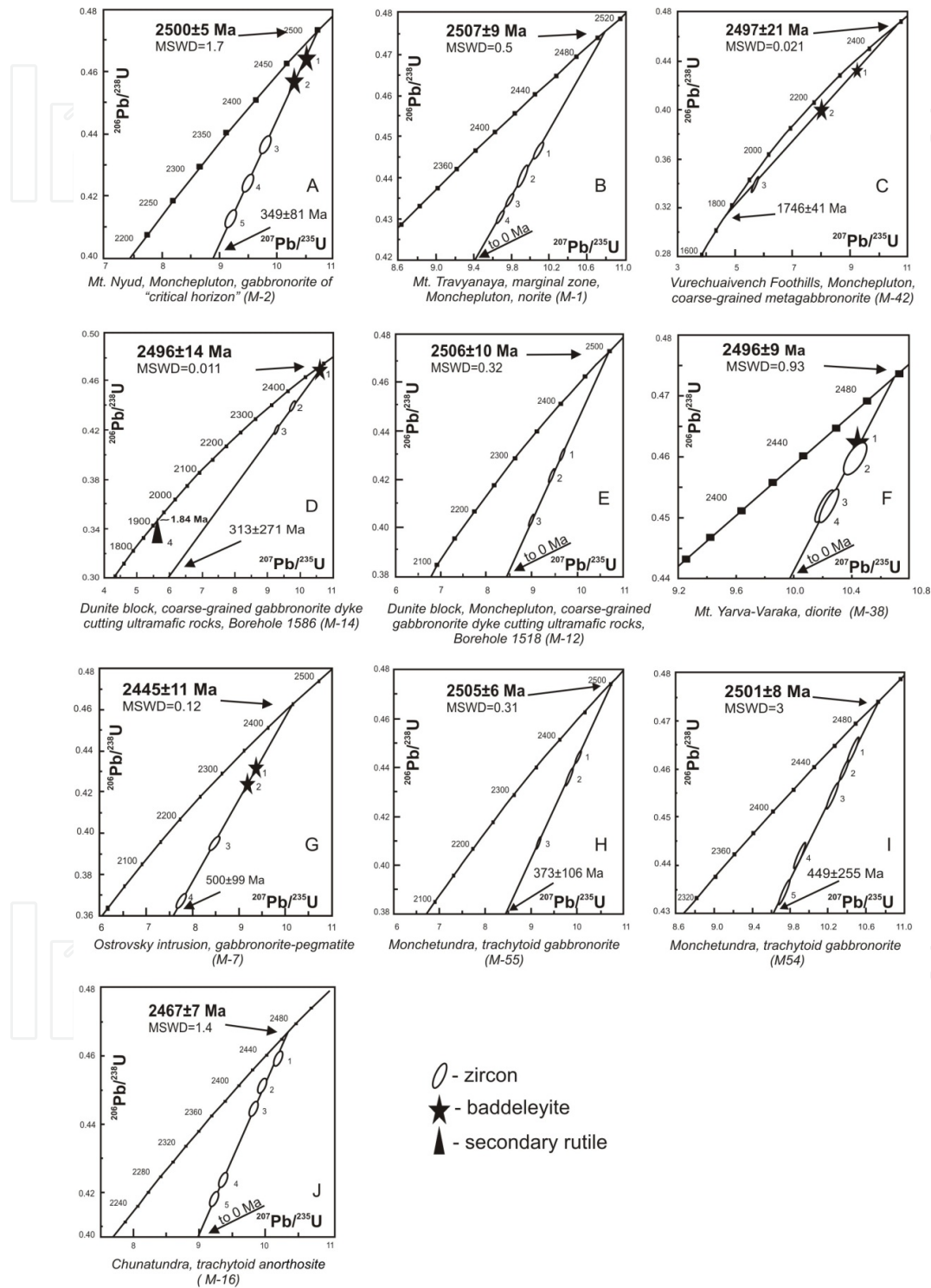
Figure 3. U-Pb concordia diagrams for zircon, baddeleyite and rutile from different rocks of the Monchegorsk Layered Complex.
