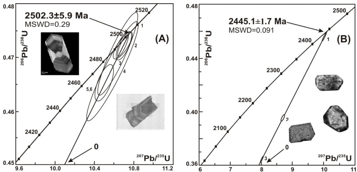
Figure 9. U-Pb concordia diagrams from Pentlandite gorge (Monchetundra massif) on: a-zircon (1-3, 6) and baddeleyite (4, 5) from plagiopyroxenite; b-zircon from gabbro-pegmatite.
