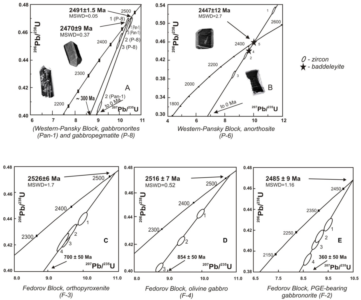
Figure 5. U–Pb concordia diagrams for the Western-Pansky (a, b) and Fedorov (c, d, e) Blocks of the Fedorovo-Pansky Complex.
