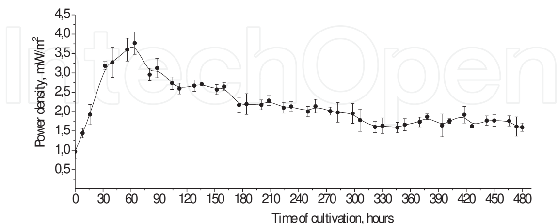
Figure 14. Power density in MFC during twenty days under addition of 9 g/l of acetic acid into the growth medium of D. acetoxidans IMV B-7384
