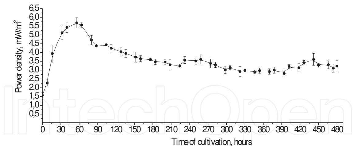
Figure 11. Power density in MFC during twenty days under addition of 6 g/l of fumaric acid into the growth medium of D. acetoxidans IMV B-7384
