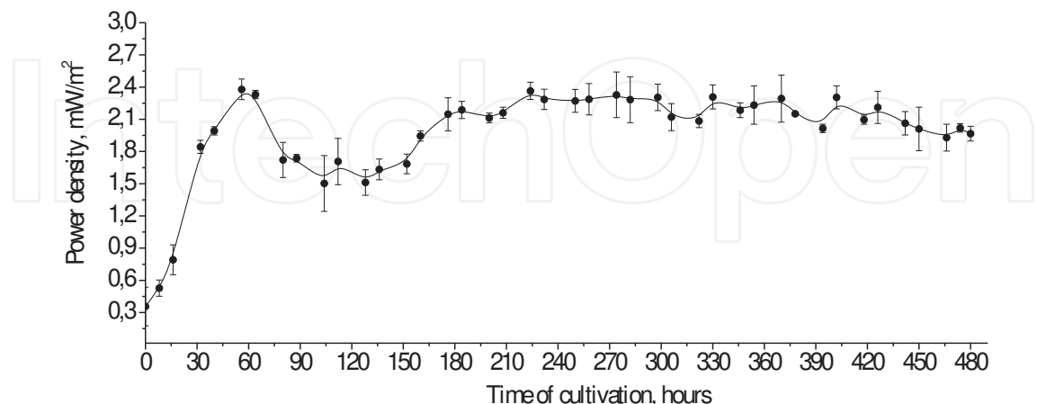
Figure 12. Power density in MFC during twenty days under addition of 9 g/l of fumaric acid into the growth medium of D. acetoxidans IMV B-7384
