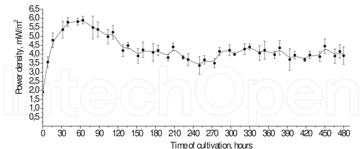
Figure 10. Power density in MFC during twenty days of D. acetoxidans IMV B-7384 cultivation under application of 9 g/l of lactic acid
