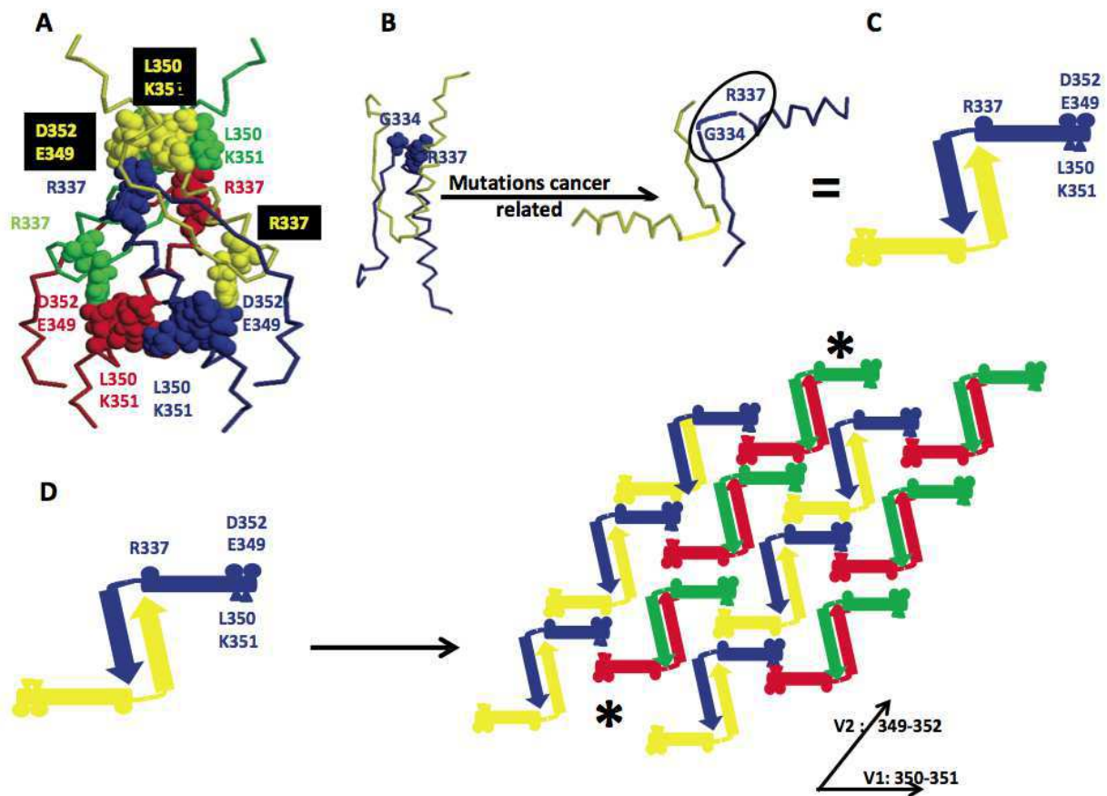
Figure 33. Transition from oligomer to fiber, the example of the p53 case. A. The p53 tetrameric domain is made of 2 dimers. Each monomer is made of a \beta -strand followed by a small helix ended by a long \alpha -helix parallel to the \beta -strand (1SAK, PDB code). The backbone of each monomer is indicated by a different color. The spacefill amino acids are the residues in contact with R337, which is a residue sensitive to mutation related to some cancer development. B. Backbone representation of the p53 dimer. The model proposes that upon mutation of R337, connections between the 2 monomers within a dimer are loosened, enabling a free movement of the long \alpha -helix relative to the \beta -strand. C. Schematic of the open-p53 dimer. D. As the structural change takes place in the four monomers, it offers enough new interfaces for growing in 2 directions \vec{V}_1 and \vec{V}_2 .
