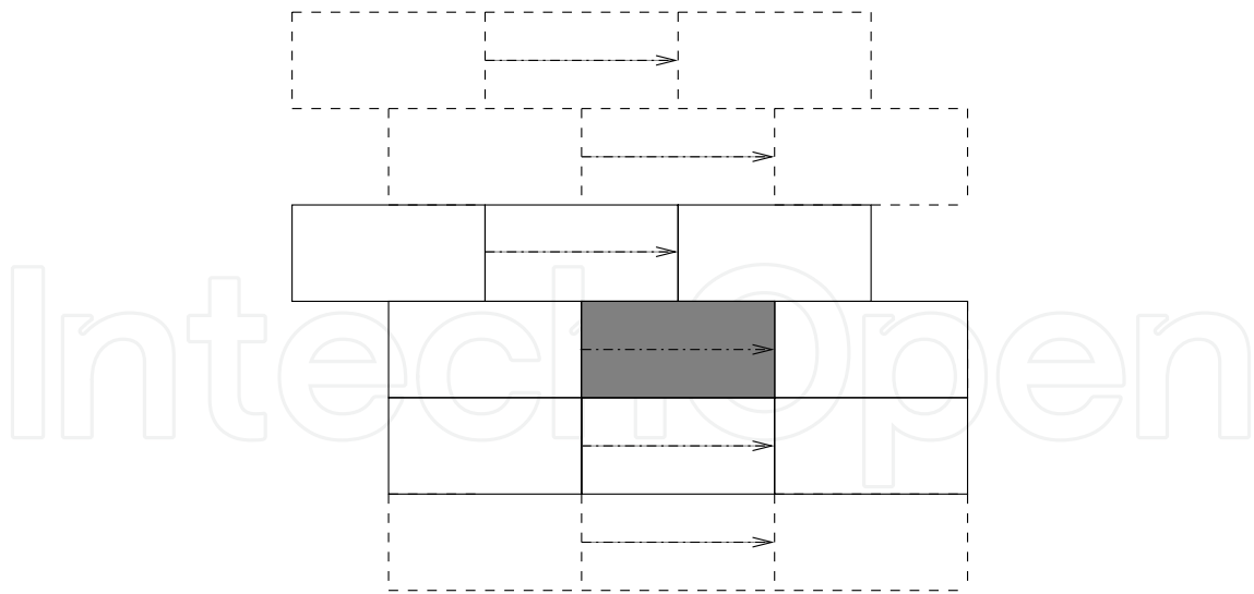
Figure 34. Non regular tiling with dominoes. The grey domino is surrounded by 5 dominoes thus this tiling is certainly not regular. Remark that the horizontal strips are invariant by the horizontal vector \vec{v}_1 and also by the vector 3\vec{v}_1 . Thus we are able to map the left border to the right border in order to form a non finite height cylinder.
