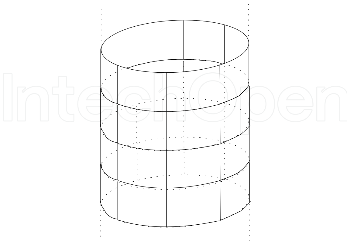
Figure 23. Fiber with a pseudo square shape. Each tile is surrounded by 4 tiles.
