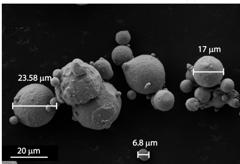
Figure 5. FESEM observation of AlSi10Mg powder.
