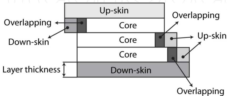
Figure 4. Up-skin, down-skin and core regions.
