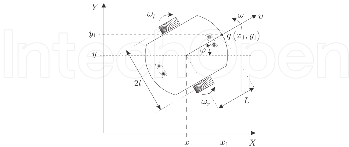
Figure 4. WMR diagram.
