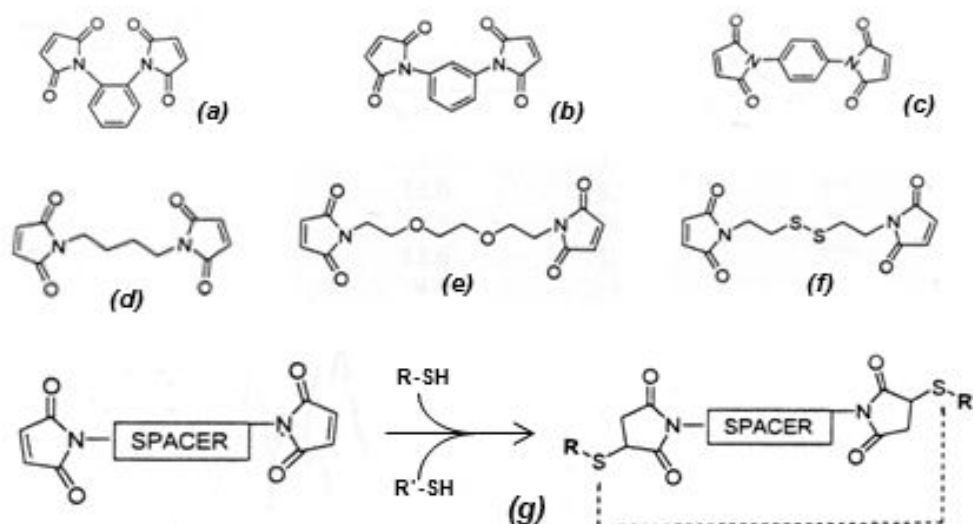
Figure 2. Some bifunctional maleimides. (a), (b), (c) ortho-meta-para N, N' phenylenemaleimide (o,m,pPDM); (d) 1,4-bismaleimidobutane (BMB); (e) 1,8-bismaleimidotriethyleneglycol (BM[PEO] 3 ); (f) dithio-bis-maleimidoethane (DMTE); (g) Reaction of a bis-maleimide derivative with sulfhydryl groups (free, reduced cysteines). Figure adapted from [20].
