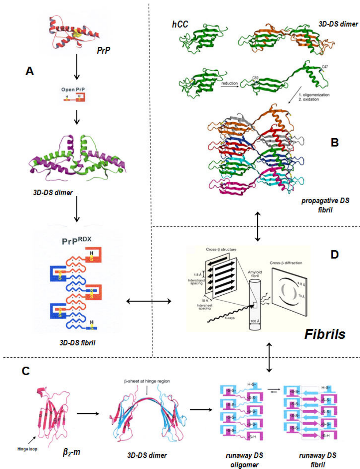
Figure 11. DS Amyloid fibrils of (A) human prion protein (hPrP), (B) human cystatin-C, hCC, and (C) \beta_2 -microglobulin ( \beta_2 -m). In all cases, fibrillogenesis is promoted by the preliminary formation of a domain-swapped dimer which evolves towards fibrils through a redox pathway. All the three fibers display the features of a generic amyloid fiber shown in panel D. The figure summarizes pictures reported in [106, 107, 110-112].
