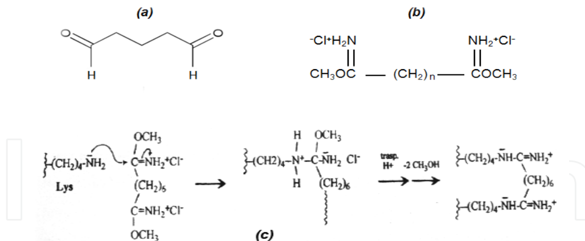
Figure 1. (a) Glutaraldehyde. (b) Diimidoesters: n=4, dimethyl-adipimidate; n=5,-pimelimidate; n=6,-suberimidate. (c) Mechanism of reaction of a protein with an imidoester (dimethylsuberimidate).
