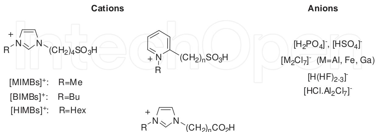
Figure 6. Cations and anions of acidic ILs
