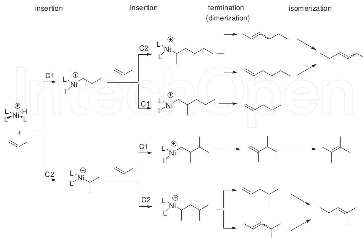
Scheme 5. Mechanism of nickel-catalyzed dimerization of propene
