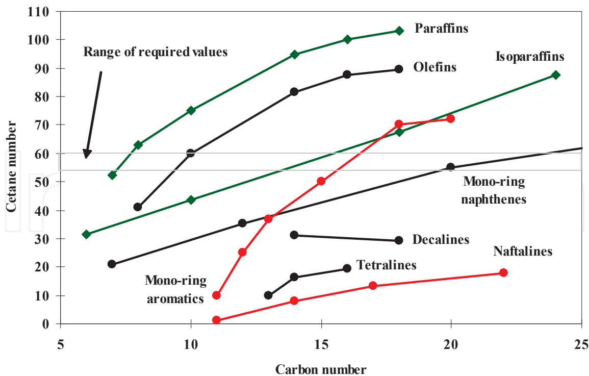
Figure 3. Cetane numbers of different hydrocarbons
