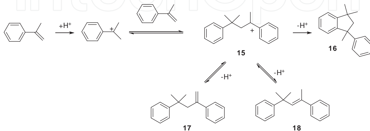
Scheme 7. Oligomerization of \alpha -methylstyrene
