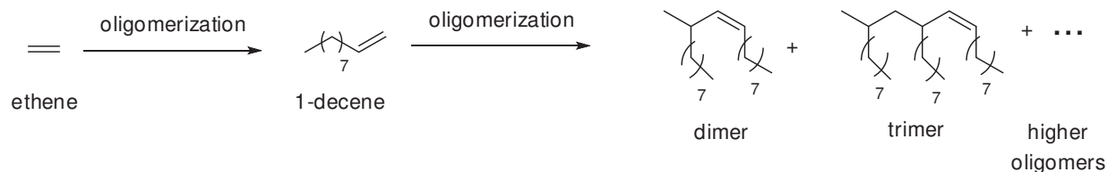
Scheme 3. Synthesis of poly- \alpha -olefins (PAOs)
