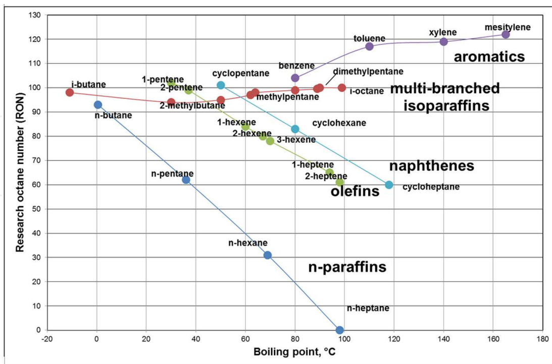
Figure 2. Research octane numbers of different hydrocarbons
