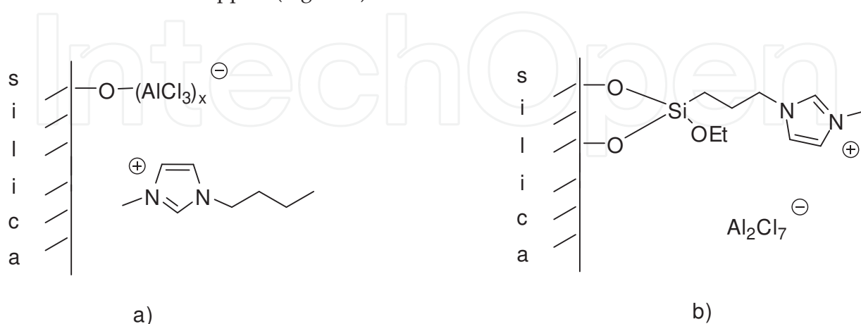
Figure 9. Structures of immobilized IL on silica support prepared by different methods (a) by mixing the IL and the silica support, b) by grafting)
