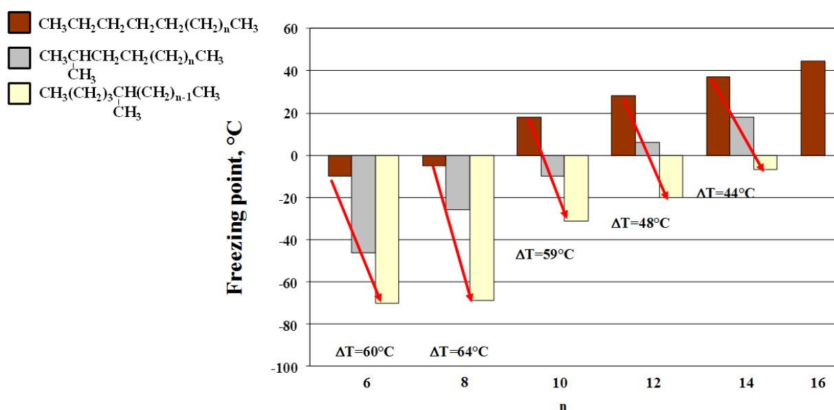
Figure 4. Freezing points of different hydrocarbons
