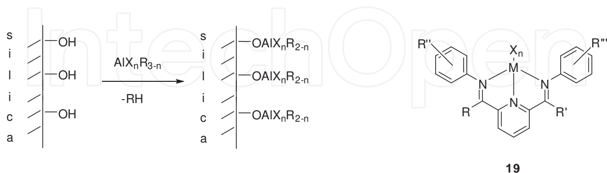
Figure 8. Modification of silica with an aluminum halide/alkylaluminum halide, and complex 19 (M=Ni, Fe, Co, Ti, V) used as the catalyst precursor
