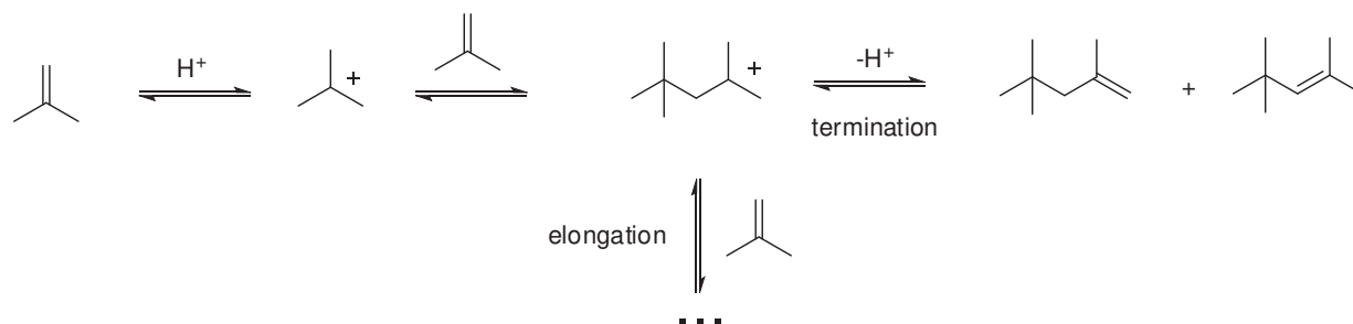
Scheme 4. Mechanism of cationic oligomerization of isobutene
