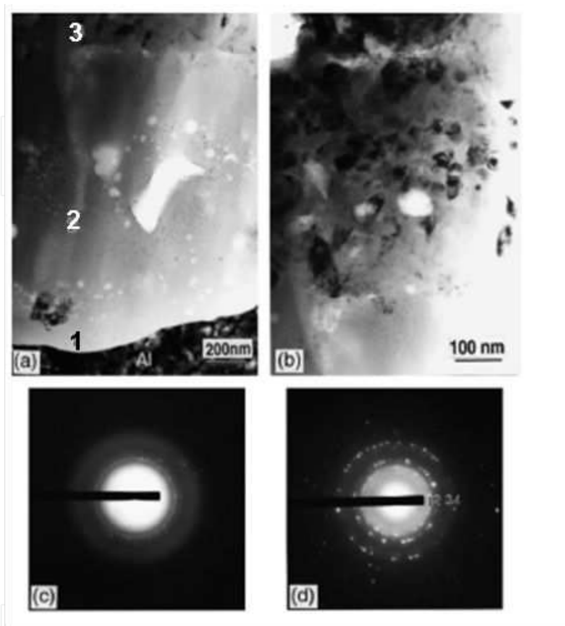
Figure 8. Cross-section TEM images of Al 6082 substrate of (a) the inner layer near coating/substrate interface and (b) the intermediate layer, and SAED patterns taken from intermediate (c) sublayer 2 and (d) sublayer 3, respectively [32].
