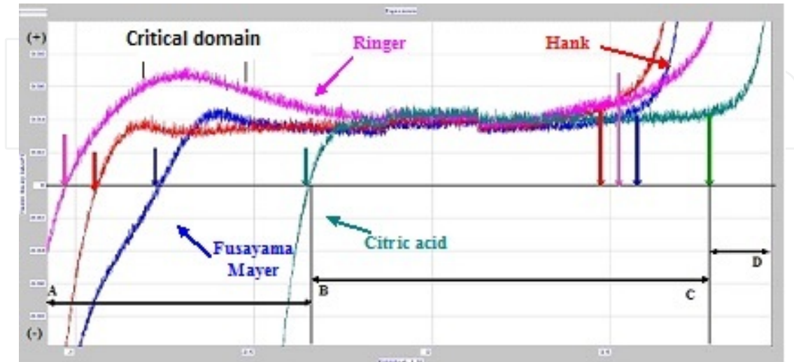
Figure 4. Identify of the passive areas on the potentiodynamic polarization curves for biomaterial Co-Cr immersed in the four environments [25, 26]
