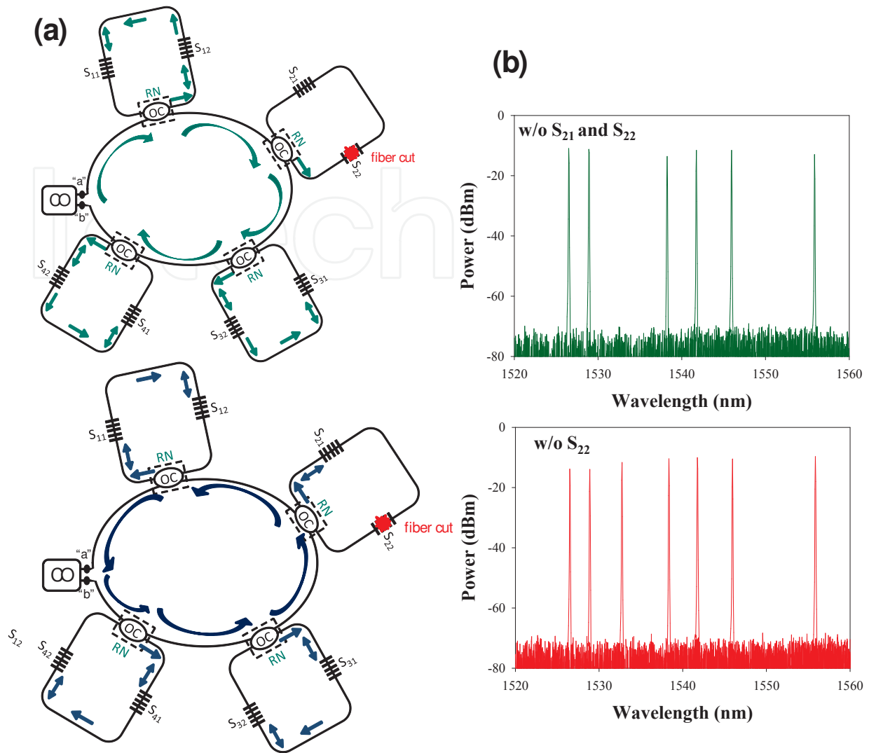
Figure 11. (a) When the sensor system has a fiber cut on the sensor S22 in the proposed sensing network. (b) Received output spectra of the eight sensing FBGs in CO. (Green and red lines represent sensing information through the path "a" and "b", respectively.)
