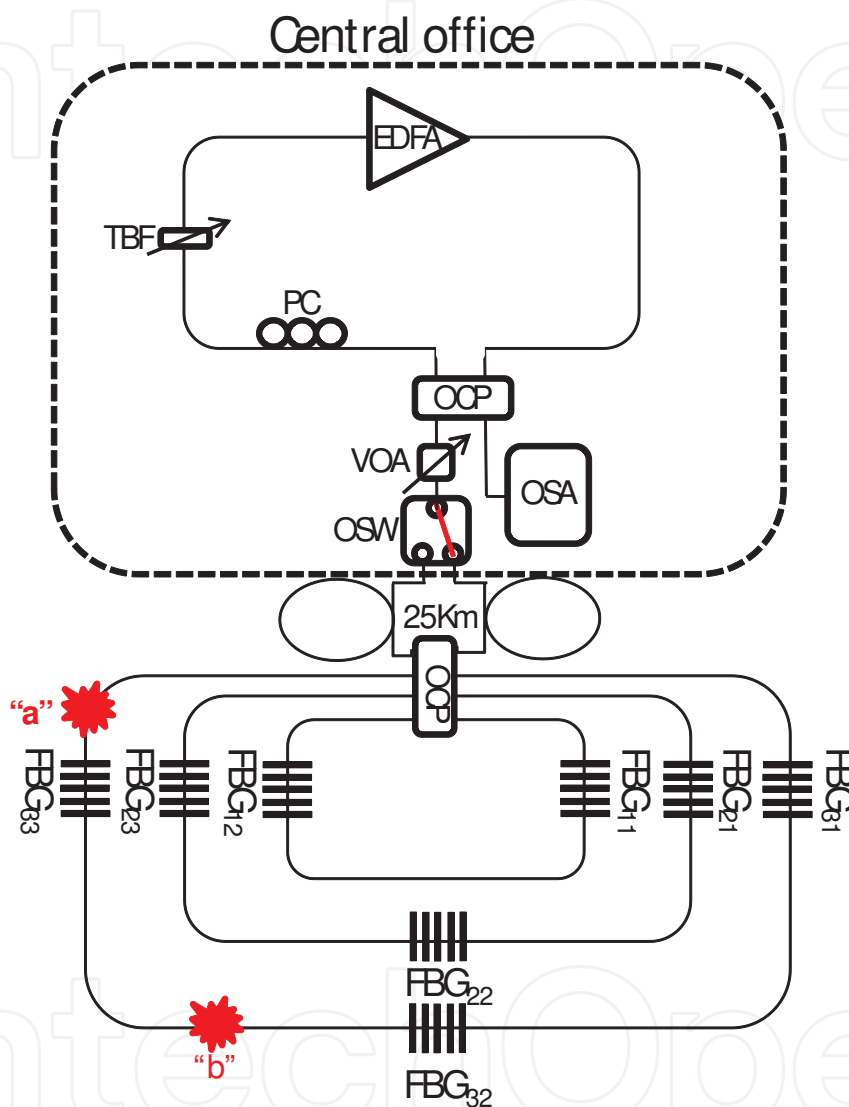
Figure 2. Experimental setup of proposed long distance self-healing FBG-based sensor system.
