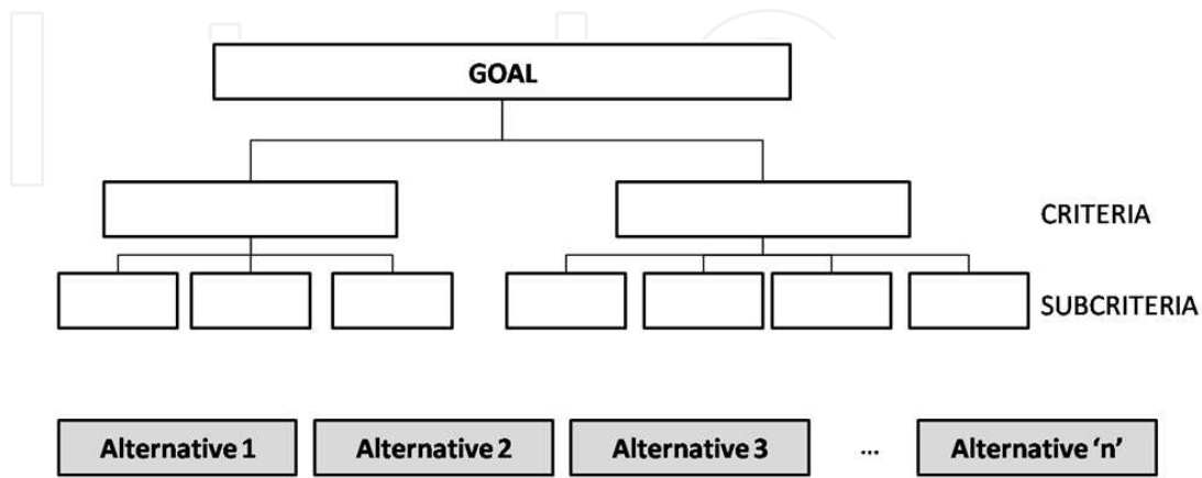
Figure 2. AHP Components: Four steps to build a hierarchy or network structure.
