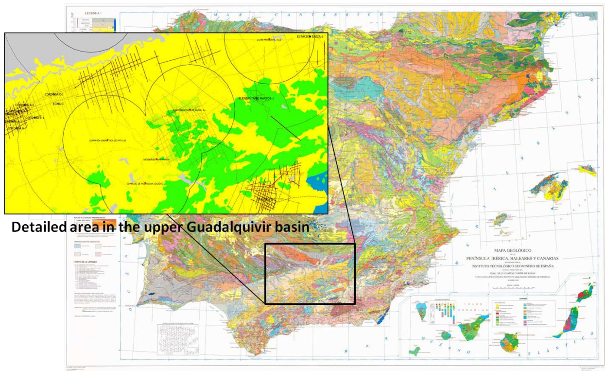
Figure 8. Spanish geological map and detailed area under evaluation. Source: IGME and AVANZA CO2 project.
