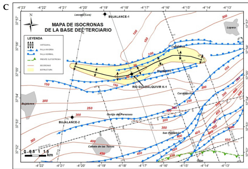
Figure 13. Detailed description of the Guadalquivir H-1 structure (called alternative C)
