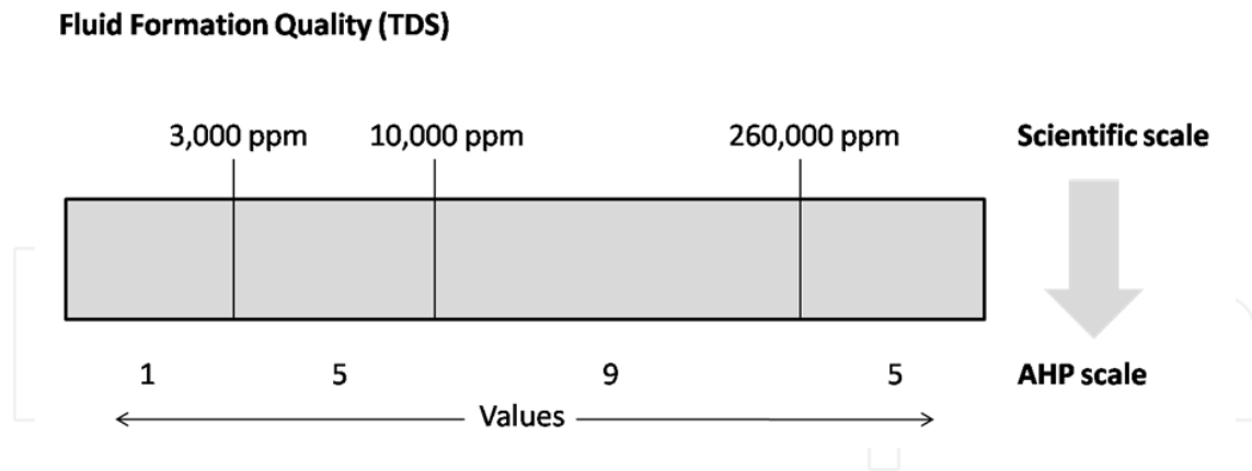
Figure 3. Scientific scale and translation into an AHP scale. This translation facilitates the evaluation of individual criteria (quantitative or qualitative) using a homogeneous scale.
