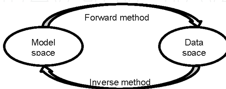
Figure 4. Connecting link between data space and model space in forward and inverse method
