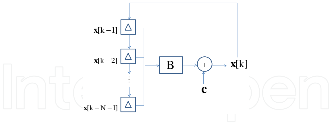
Figure 2. A linear recurrent system for synchronous computations. The triangle denotes time delay.
