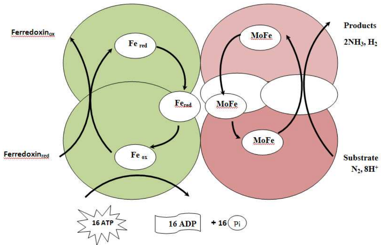
Figure 3. The structure of nitrogenase
