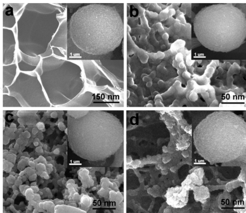
Figure 5. SEM images of the surface of the regenerated cellulose microspheres (RCS) (a), M10 (mixed solutions of \text{FeCl}_3/\text{FeCl}_2 with concentration of 10mmol/5.2mmol) (b), M20(mixed solutions of \text{FeCl}_3/\text{FeCl}_2 with concentration of 20mmol/10.6mmol) (c) and M30(mixed solutions of \text{FeCl}_3/\text{FeCl}_2 with concentration of 30mmol/15.9mmol) (d). The insert illustrates the morphology of RCS and magnetic regenerated cellulose microspheres (MRCS).
