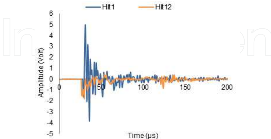
Figure 4. AE waveform for two different AE amplitudes during sensitivity checking
