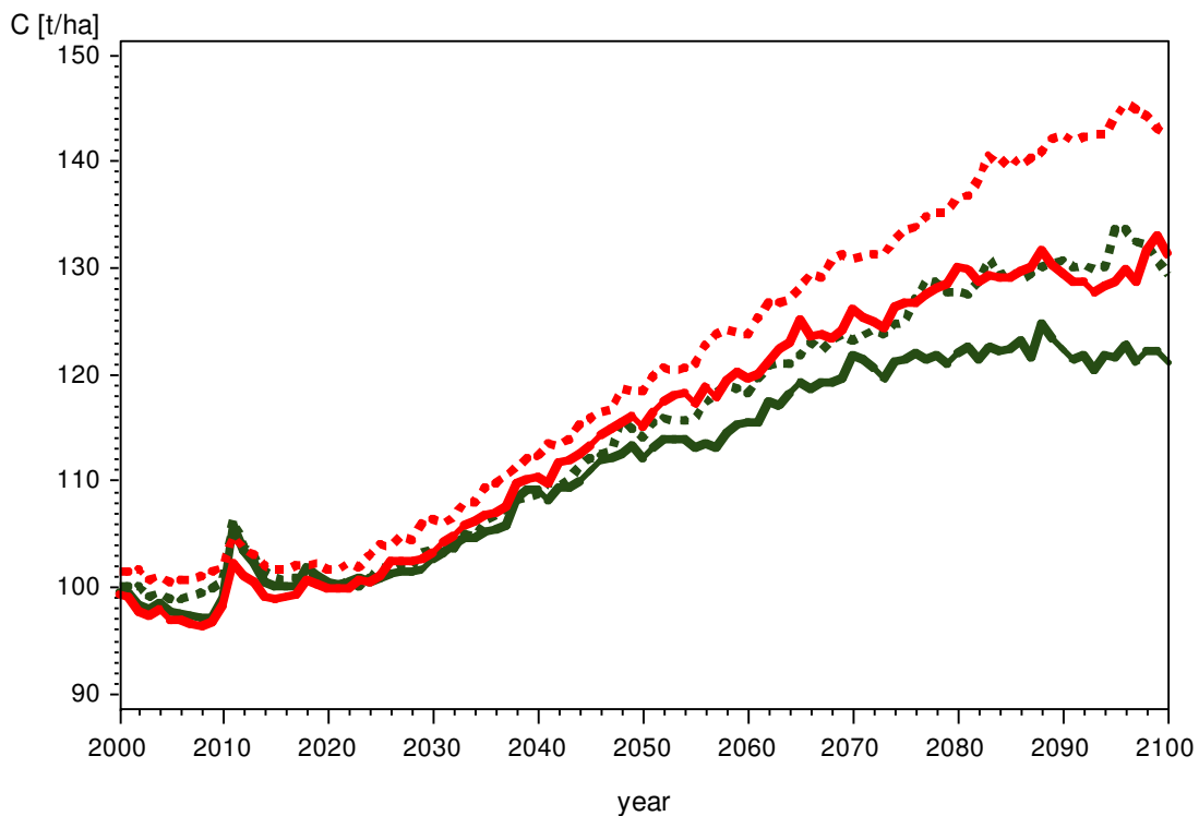
Figure 4. Simulated temporal trend of the soil carbon stock (C [ton/ha]) for an example stand in the Ossiacher Tauern between the year 2000 and 2100. Red: beech dominated forest, green: spruce dominated forest; full lines: climate scenario A1B; dashed lines: climate scenario B1.
